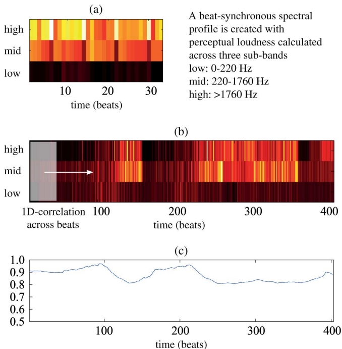
Fig. 5. Spectral balance overview. (a) beat synchronous spectral representation for input phrase section, (b) the beat synchronous spectral representation for the candidate song, and (c) the spectral balance per beat shift, M_{L,n}(k) .
