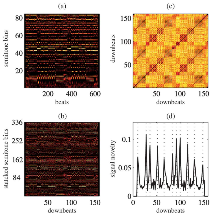
Fig. 1. Phrase-level segmentation overview. (a) a beat synchronous tuned semitone spectrogram. (b) a downbeat-synchronous spectrogram, where groups of four beat frames are stacked into bars. (c) a self-similarity matrix generated from the downbeat-synchronous semitone spectrogram. (d) a novelty function whose peaks highlight likely phrase boundaries. The vertical dotted lines show the detected phrase boundaries.
