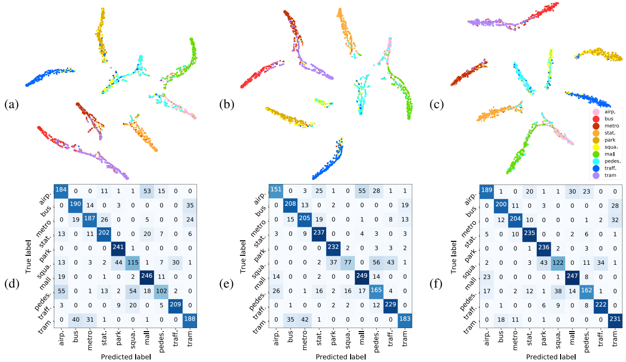
Fig. 3. Visualization of the learned representations using t-SNE [37]. Subplots (a), (b), and (c) are the output of the scene classification layer in MoE-AST , Mihe-AST , and cSEM-AST on TUT2018 test set, respectively. Subplots (d), (e), and (f) are the corresponding confusion matrix of (a), (b), and (c), respectively.
