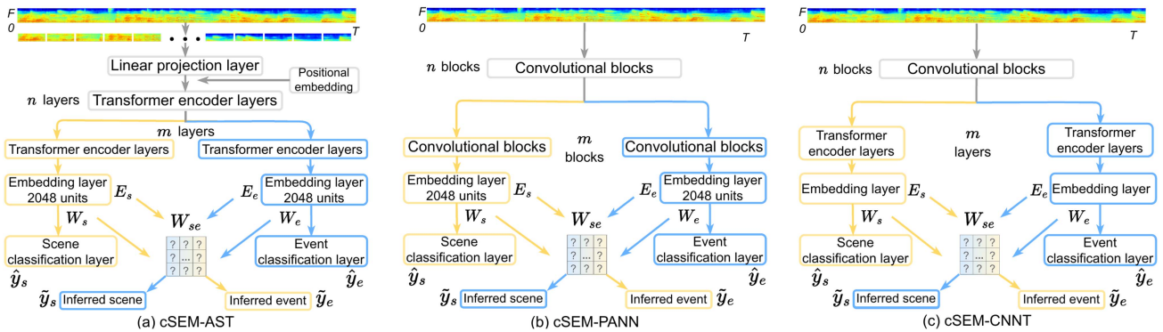
Fig. 2. Models based on the proposed cSEM framework.
