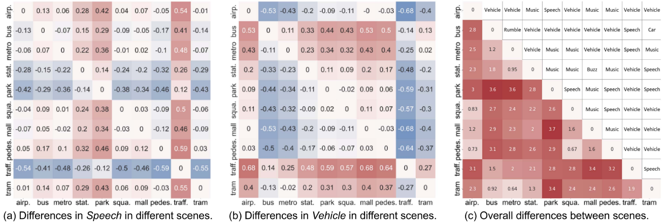
Fig. 5. Differences between acoustic scenes on the development set of TUT2018, where subplots (a) and (b) take the audio event Speech and Vehicle as examples, while subplot (c) shows the overall differences between scenes.
