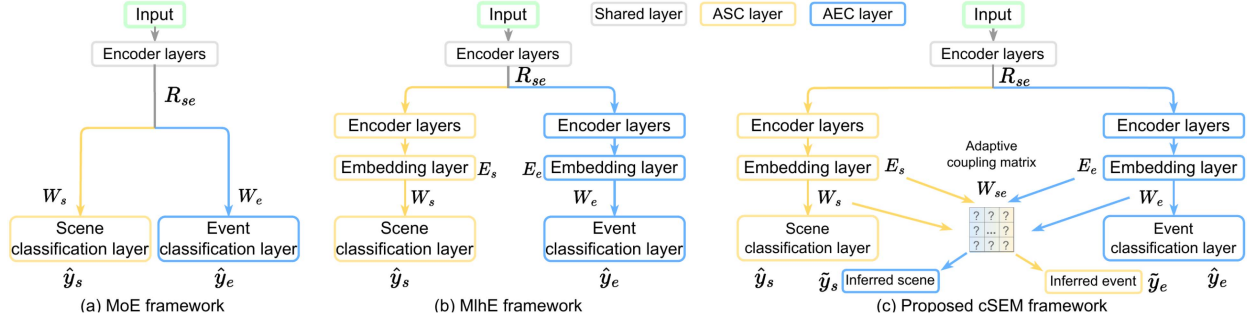
Fig. 1. Three frameworks for scene-event joint modelling: (a) MoE: modelling using the same one embedding space; (b) MlhE: modelling using shared low-level and separated high-level embedding spaces; (c) cSEM: the proposed cooperative scene-event modelling with adaptive coupling matrix.
