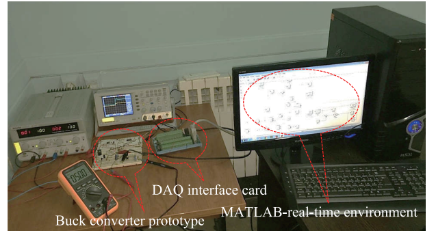
Fig. 4. Experimental prototype.
