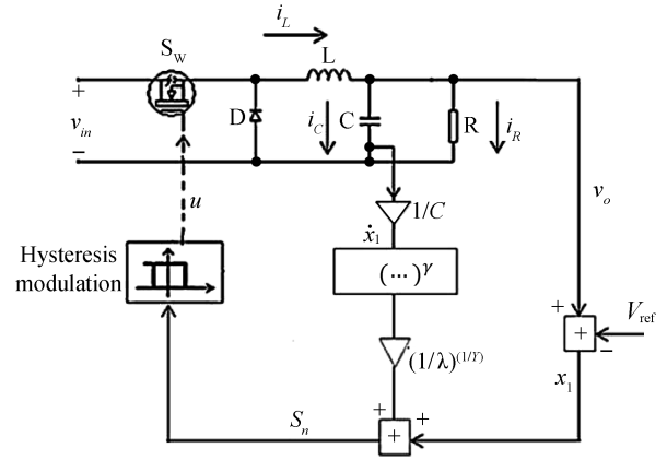
Fig. 3. Buck converter control system block diagram using NTSMC.
