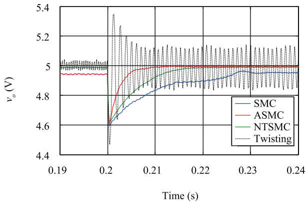
Fig. 20. The output voltage diagrams by different sliding mode methods during changes in load resistance from 10\Omega to 2\Omega at t = 0.2\text{s} .
