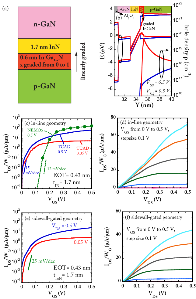
FIGURE 4. (a) Epitaxial structure and (b) computed band diagram and hole density (red line) of GaN/InN/graded-InGaN/GaN inline TFET heterostructures, where the InN thickness is 1.7 nm and graded InGaN is 0.6-nm thick. GaN/InN/GaN abrupt inline TFET band diagram and hole density (blue line) are also included for comparison. (c) Transfer and (d) output characteristics for a graded inline TFET. (e) Transfer and (f) output characteristics for a sidewall-gated TFET based on the epitaxial structure in (a). In (c), the solid lines are from TCAD simulations, while the dashed lines with dots are from NEMO5.
