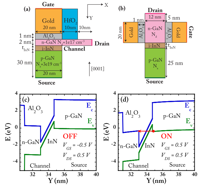
FIGURE 2. TFETs based on GaN/InN/GaN heterojunction. (a) Inline design, (b) sidewall-gated design, (c) OFF-state band diagram, and (d) ON-state band diagram for an inline TFET. The doping concentrations shown are the physical impurity concentrations.
