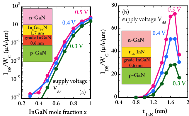
FIGURE 6. Inline TFET ON-current dependence on (a) InGaN interlayer In mole fraction and (b) InN layer thickness at supply voltages of 0.3, 0.4, and 0.5 V. Insets: corresponding heterojunction epitaxial structures. The calculated results shown in the figures are from TCAD simulations.
