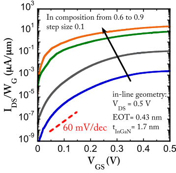
FIGURE 5. Transfer characteristics for inline TFET based on GaN/In x Ga 1-x N/graded-InGaN/GaN heterojunction, with In mole fraction from 0.6 to 0.9. The calculated results are from TCAD simulations.
