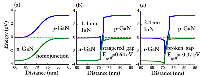
FIGURE 1. Computed band diagrams for (a) GaN homojunction, (b) staggered-gap GaN/InN/GaN heterojunction with 1.4-nm InN layer thickness, and (c) broken-gap GaN/InN/GaN heterojunction with 2.4-nm InN layer thickness.
