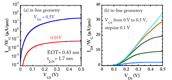
FIGURE 3. (a) Transfer and (b) output characteristics for an inline TFET based on an abrupt GaN/InN/GaN heterojunction.
