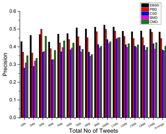
Fig. 10. Comparison of precision values of several algorithms.
