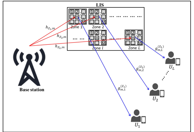
Fig. 1. LIS-based NOMA system model with L users.
