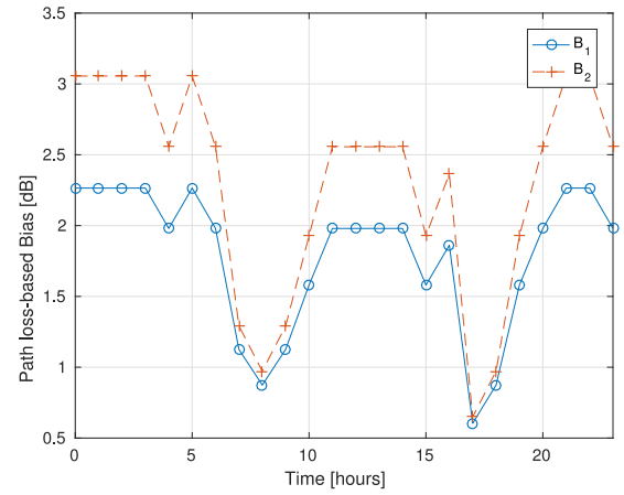
Fig. 9. Optimal handover bias throughout the day for January 23, 2015.
