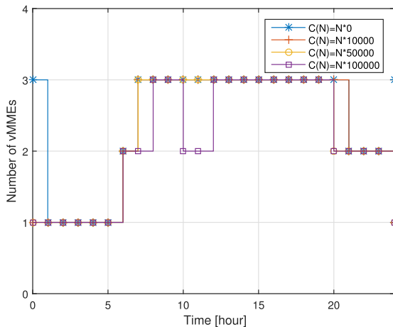
Fig. 13. N_{\text{opt}} for different costs C(N) , during January 23, 2015.
