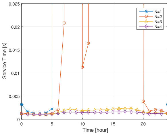
Fig. 11. Average service time \tau for different N , during January 23, 2015.
