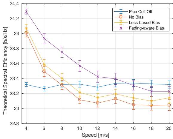
Fig. 8. Theoretical spectral efficiency as a function of the vehicular traffic speed v .
