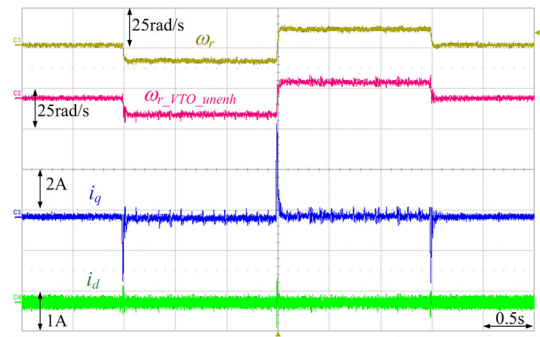
Fig. 16. Low-speed no-load command tracking when the drive is equipped with a 1 BPP position sensing system.
