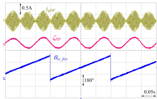
Fig. 11. Blocked rotor no-load high-frequency pulsating signal-injection test.
