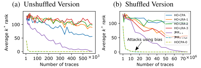
FIGURE 5. Comparison of different attacks' guessing entropies on the secured ANSSI's AES.
