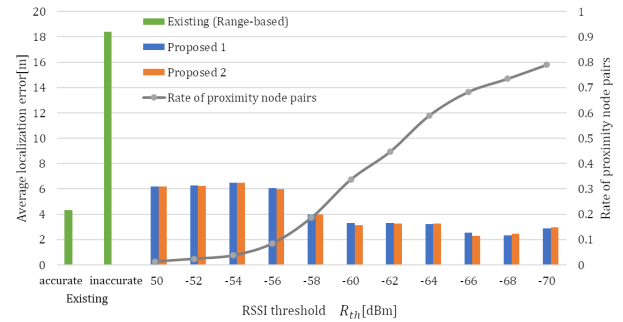
FIGURE 10. Results obtained in real-world laboratory environment.
