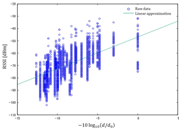
FIGURE 8. Parameter estimation results for situation B.
