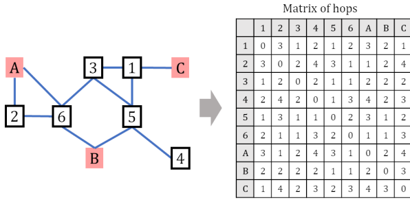
FIGURE 3. Graph representing the proximity relation of nodes (left) and the matrix of hops (right).
