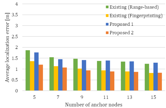
FIGURE 16. Comparison results of the number of anchor nodes effects obtained when the attenuation model is accurate.
