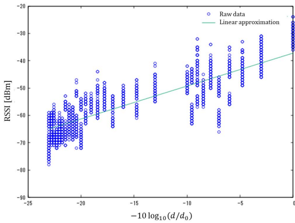
FIGURE 7. Parameter estimation results for situation A.
