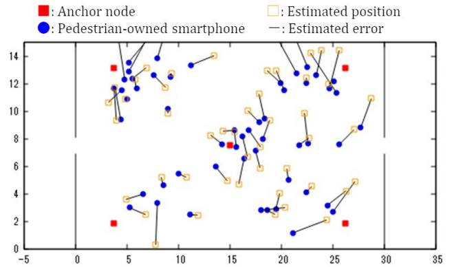
FIGURE 12. Example localization result obtained by proposed method 2. The average localization error was 1.2 m.
