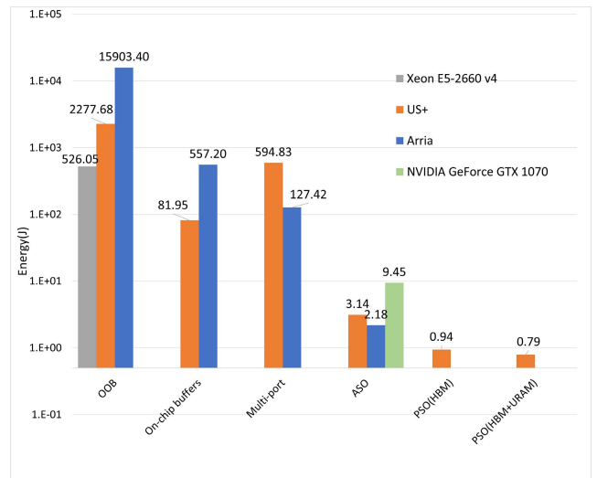
FIGURE 11. Energy utilization on target platforms (log scale).
