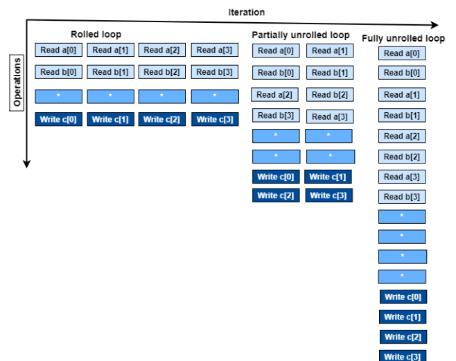
FIGURE 6. Loop unrolling/vectorization.
