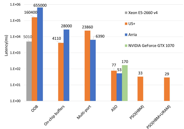
FIGURE 8. Average latency (log scale).
