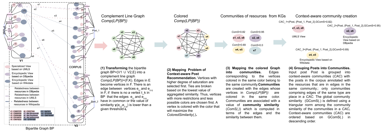
FIGURE 3. Running Example. Mapping the Problem of Context-Aware Post Recommendation into the Vertex Coloring Problem. Entities in a post are annotated with terms in different contexts (e.g., domain-specific or encyclopedic), relatedness between the terms in the same context are represented by edges of a Bipartite Graph BP=(V_1 \cup V_2, E) ; a similarity measure quantifies relatedness of the terms in a context. (1) The complement of the line graph of BP is computed Comp(LP(BP))=(F, K) . (2) Comp(LP(BP))=(F, K) is colored with the minimal number of colors that maximize the value of ColoredSimilarity(.) . (3) Colored Graph in mapped into Communities. (4) Communities are used to create Context-Aware Communities of Posts.
