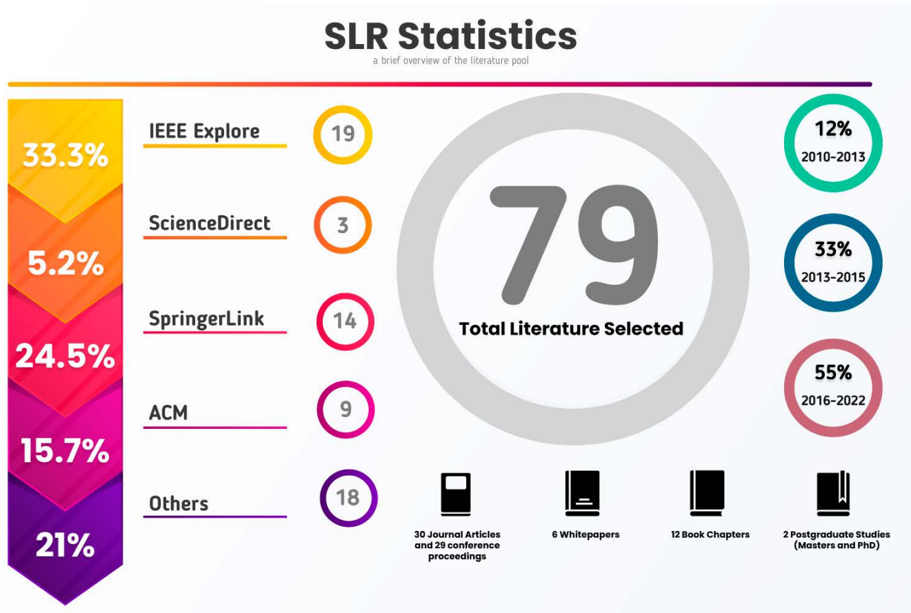
FIGURE 2. SLR Statistics.
