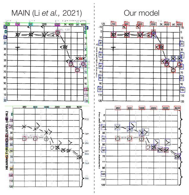
FIGURE 8. Comparison of the components detected within representative audiograms. The axis labels and audiological symbols detected by Li et al.'s model (left) and ours (right) within two representative audiograms used for testing. The colors of the boxes on the left represent the different classes of objects. For our model, blue boxes represent label detections on the hearing loss axis or left ear symbols, while red boxes represent label detections on the frequency axis or right ear symbols.
