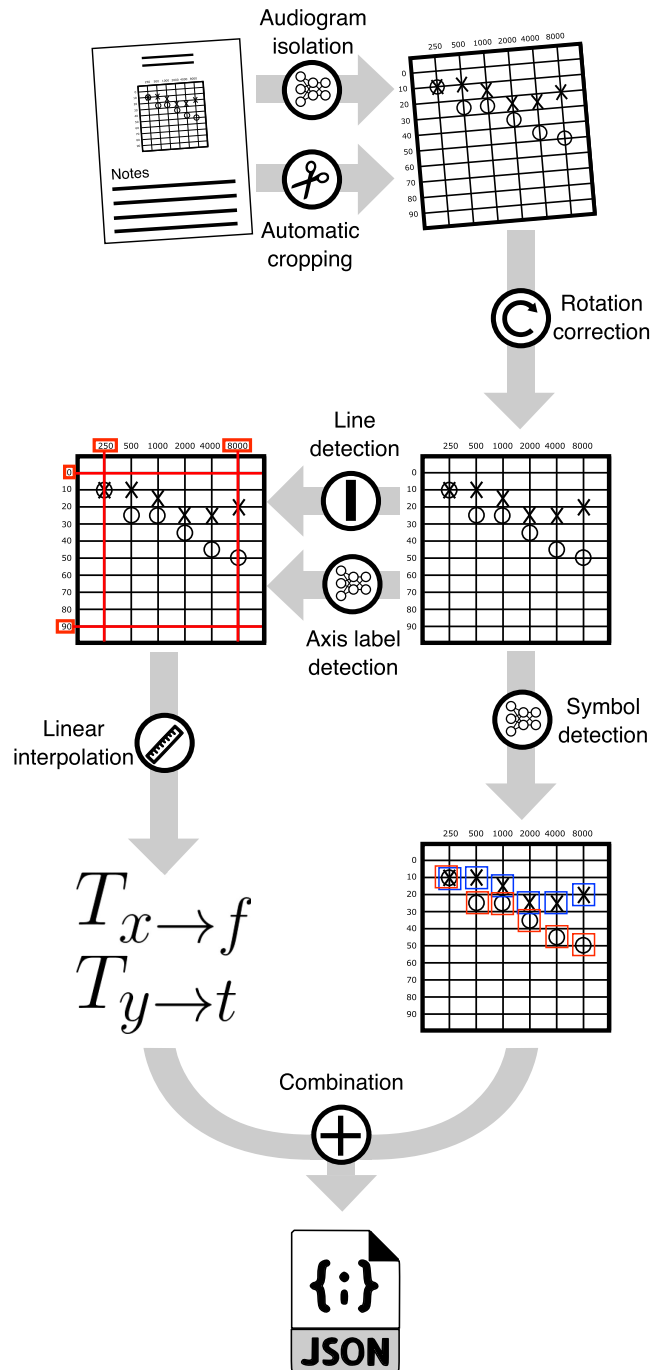
FIGURE 2. Audiogram digitization strategy. Our strategy combines a series of deep learning-based object detection tasks with traditional image processing procedures (line detection, cropping, rotation). These steps enable the derivation of pixel-to-frequency and pixel-to-threshold transforms through linear interpolation. These transforms are subsequently applied to the pixel coordinates of detected audiological symbols to generate a JSON document listing the individual hearing thresholds.
