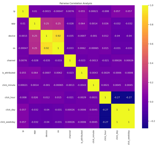
FIGURE 10. Correlation analysis of temporal patterns with respect to target attribute.
