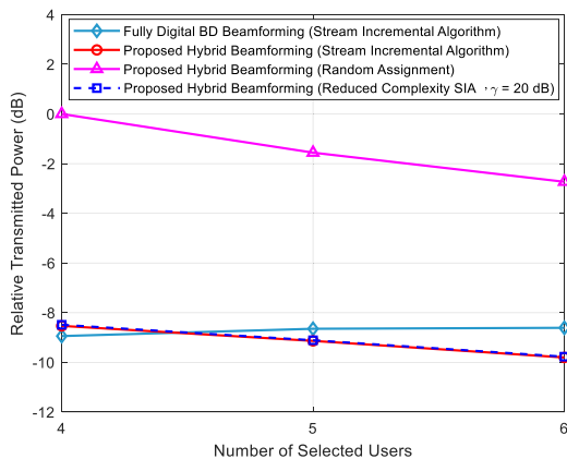
FIGURE 9. Relative transmitted power versus the number of selected users of different methods for the 192 \times 16 OFDM MIMO system; N_{tRF} = 8 , N_s = 8 , N_{rRF} = 3 , and system sum rate = 39.2 Mbps.
