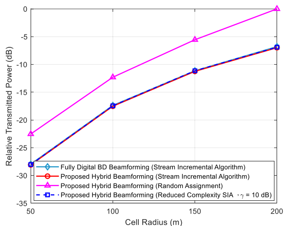
FIGURE 4. Relative transmitted power versus cell radius of different methods for the 128 \times 16 OFDM MIMO system; four users, N_{tRF} = 5 , N_s = 5 , and N_{rRF} = 3 .
