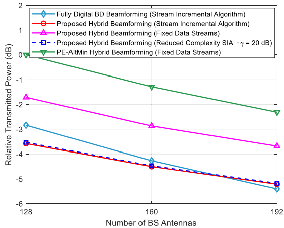
FIGURE 8. Relative transmitted power versus the number of BS antennas of different methods for the OFDM MIMO system, four users, N_{tRF} = 8 , N_s = 8 , and N_{rRF} = 3 .
