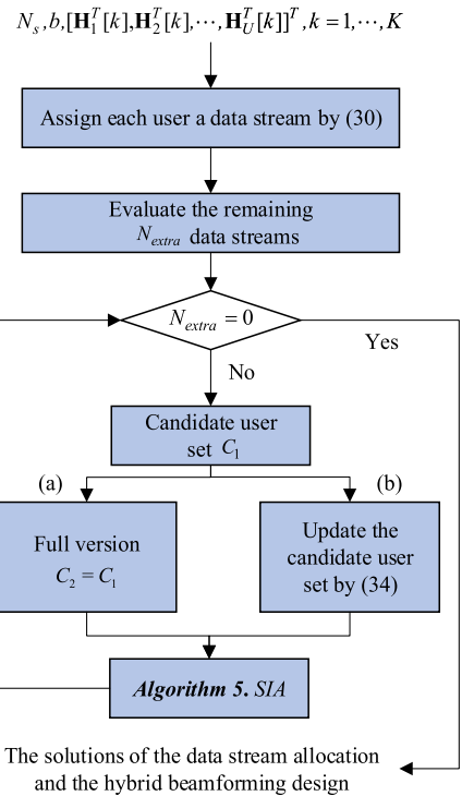
FIGURE 2. Flow chart of the proposed processing scheme.
