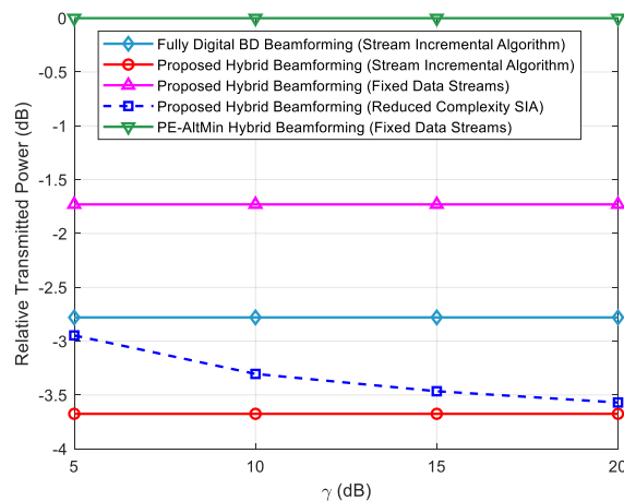
FIGURE 6. Relative transmitted power versus \gamma of different methods for the 128 \times 16 OFDM MIMO system, four users, N_{tRF} = 8 , N_s = 8 , and N_{rRF} = 3 .
