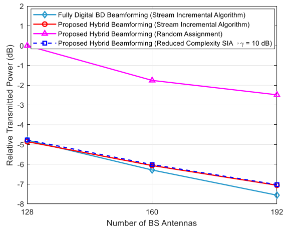
FIGURE 5. Relative transmitted power versus the number of BS antennas of different methods for the OFDM MIMO system; four users, N_{tRF} = 5 , N_s = 5 , and N_{rRF} = 3 .
