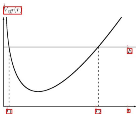
FIG. 1: The shape of our potential V_{eff}(r) with \eta > 0 .
