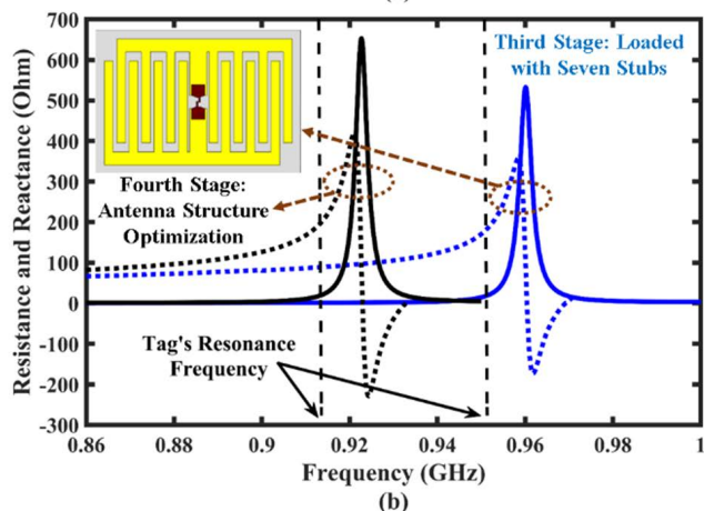
FIGURE 2. Input impedance of the tag antenna at (a) the first (loaded with three identical open stubs) and second stages (loaded with five identical open stubs), (b) the third (loaded with seven identical stubs) and final stages (tuning the dimensions of the antenna). (Solid line: resistance, dotted line: reactance).
