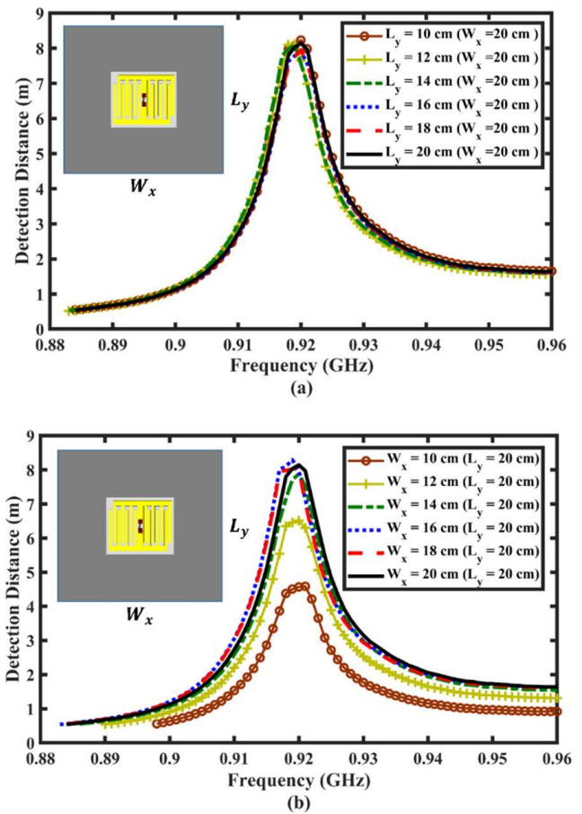
FIGURE 9. Measured detection distance of the suggested tag at various dimensions of (a) L_y from 10 cm to 20 cm for fixed W_x and (b) W_x from 10 cm to 20 cm for fixed L_y .
