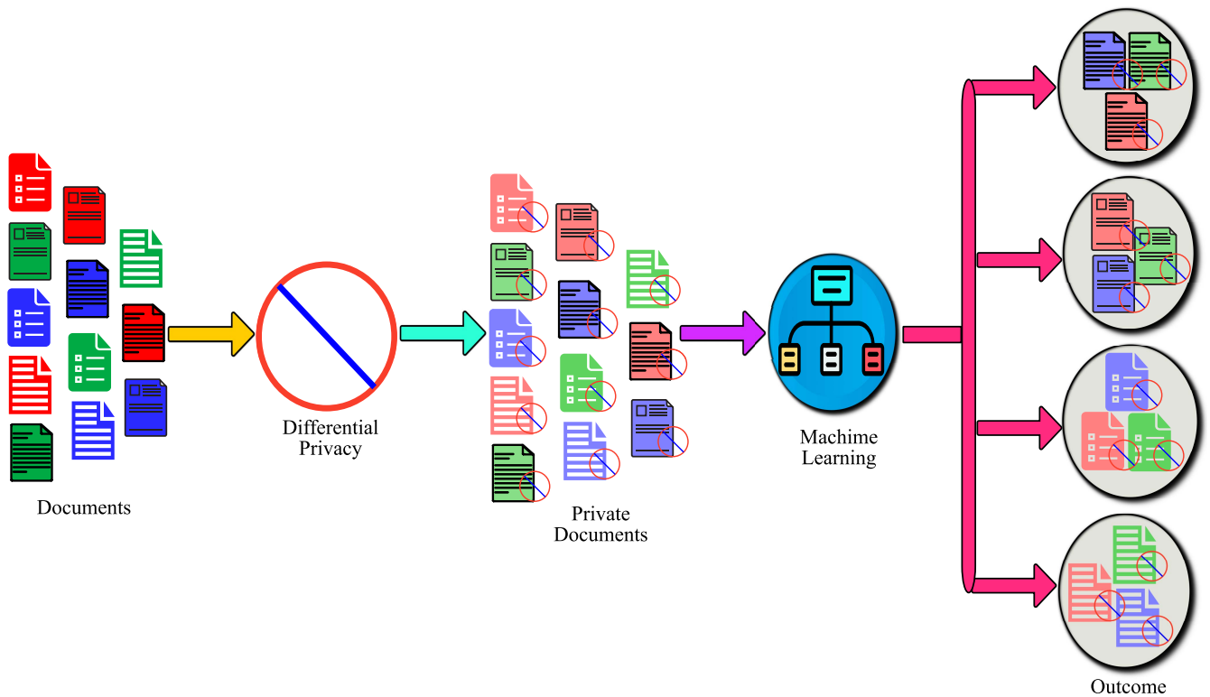
FIGURE 5. Standard model for differential privacy with machine learning.
