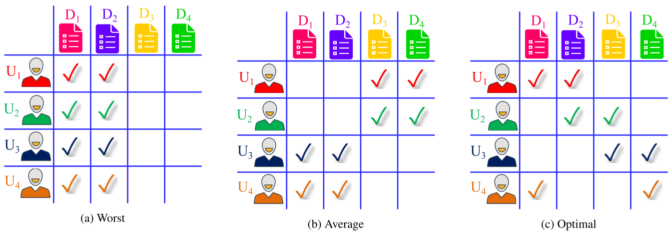
FIGURE 7. Distribution Strategy (a) W_j^* = W_k^* (b) minimize \sum_{j \neq k} |W_j^* \cap W_k^*| (c) minimize \sum_j \frac{1}{|W_j^*|} \sum_{k \neq j} |W_j^* \cap W_k^*| .
