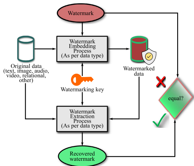
FIGURE 6. Key components of watermarking based models.
