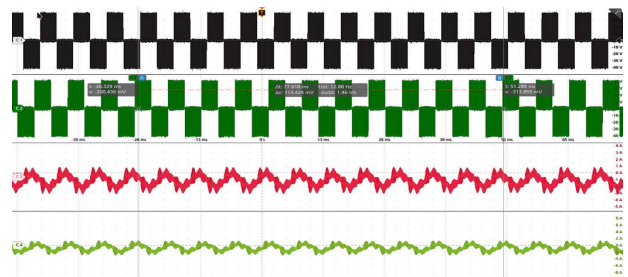
FIGURE 42. Phase current and line-line voltage waveform at 750 rpm.
