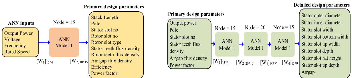
FIGURE 52. E-motor deign ANN model 1 and ANN model 2.
