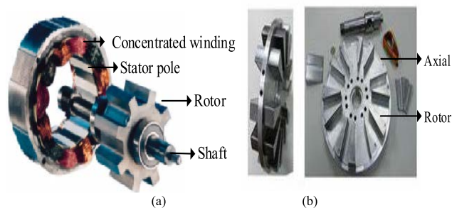
FIGURE 25. (a) SRM radial flux. (b) SRM axial sandwiched with rotor.
