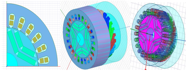
FIGURE 16. (a) FEA Analysis PMASynRM. (a) 2D. (b) 3D. (c) Rotor flux density.
