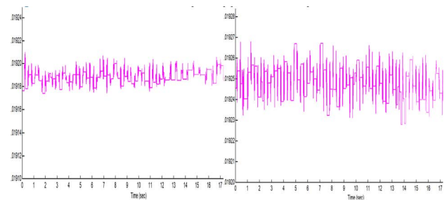
FIGURE 46. TSF-DITC and DTC torque ripple at 5700 rpm.
