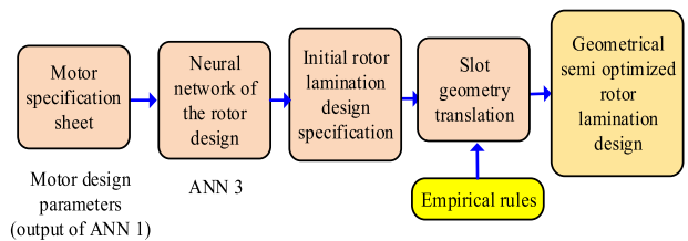
FIGURE 53. E-motor deign ANN model 3.
