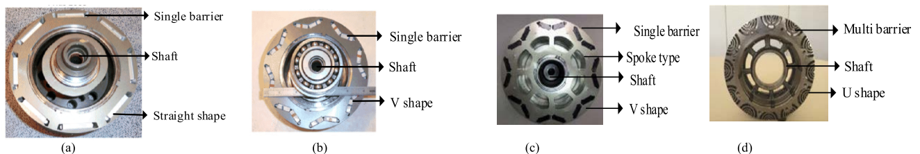
FIGURE 17. Four generation e-motors Prius. (a) 2004 Prius PM split, 33 kW, 274 VDC, 6 krpm. (b) 2004 Prius single-V, 50 kW, 500 VDC, 6 krpm. (c) 2016 Chevy Volt IPM motor, 60 kW, 650 VDC, 13 krpm. (d) 2017 Prius surface grooves 53 kW, 580 VDC, 17 krpm [99].
