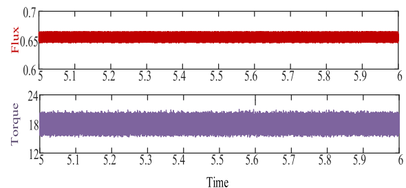
FIGURE 41. FOC fed torque and flux response at 750 rpm.
