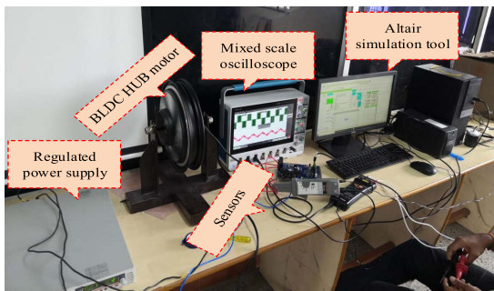
FIGURE 39. Hardware BLDC hub type motor setup.
