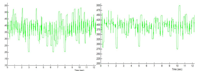
FIGURE 40. DTC and intelligent control torque ripple at 750 rpm.
