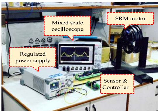
FIGURE 44. SRM hardware setup.
