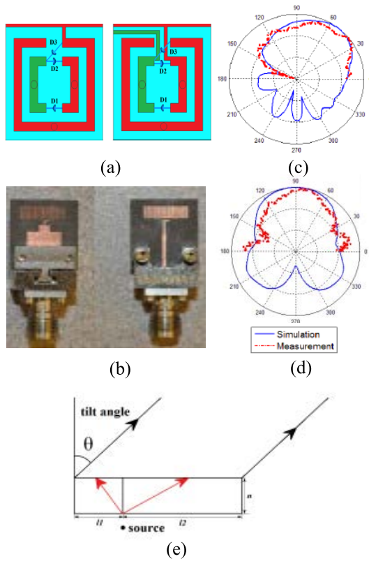
FIGURE 13. The dipole antenna of [145] with the reconfigurable SRR: (a) top and bottom views of the reconfigurable SRR, (b) the fabricated dipole antenna loaded by an array of SRRs, (c) and (d) the simulated and measured radiation patterns in E-plane and H-plane, respectively, (e) the beam deflection mechanism.
