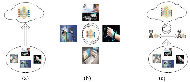
FIGURE 7. Architecture modes of distributed training. (a) Centralized; (b) Decentralized; (c) Hybrid.
