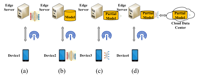
FIGURE 8. EI inference models. (a) Edge-based mode; (b) Device-based mode; (c) Edge-device mode; (d) Edge-cloud mode.
