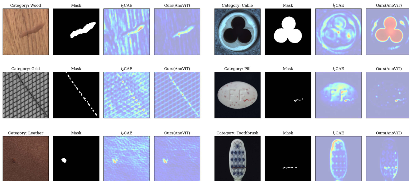
FIGURE 3. Qualitative result of anomaly localization in MVTecAD.
