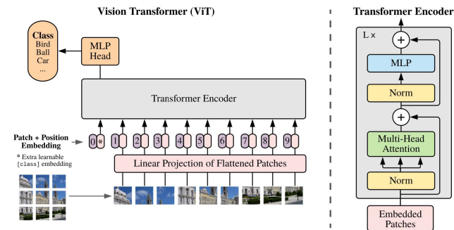
FIGURE 1. Architecture of original ViT.
