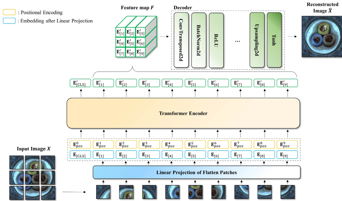
FIGURE 2. Architecture of AnoViT.
