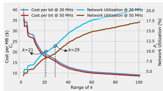
FIGURE 6. Cost per MB ( C_v ) and potential network utilization ( P_v ) as a function of k for two bandwidth scenarios of B = [30, 50] , respectively. The appropriate range of k (21 to 29) is shown by the dotted lines.
