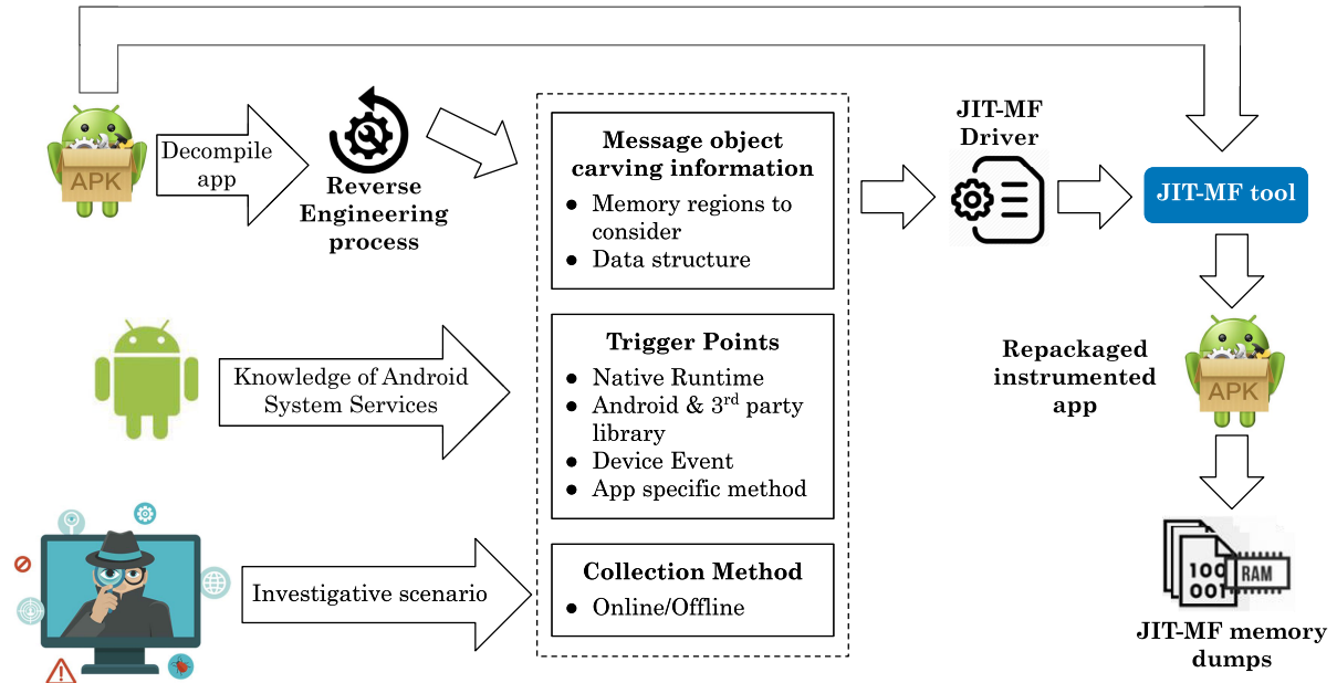
FIGURE 5. JIT-MF drivers.
