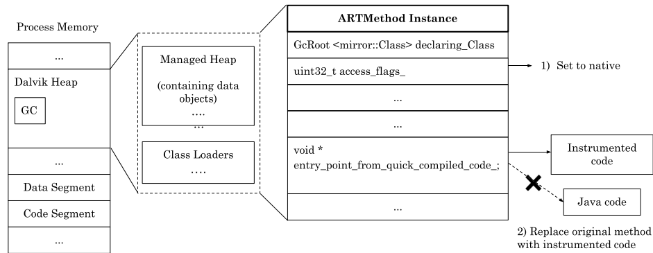
FIGURE 4. Instrumenting code via ArtMethod entry point.
