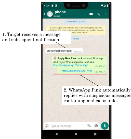
FIGURE 11. WhatsApp pink attack steps.
