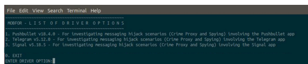
FIGURE 10. MobFor JIT-MF driver selection screen.
