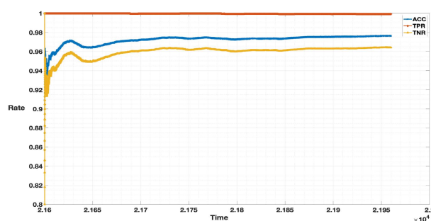
FIGURE 18. The community accuracy with the true positives and negatives rates.
