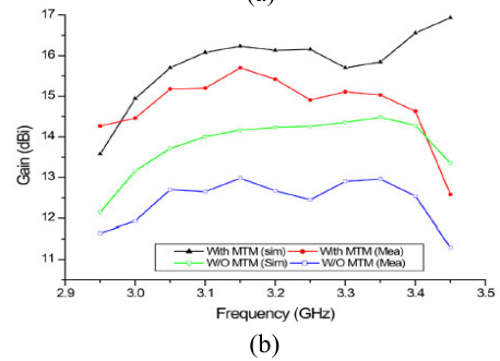
FIGURE 13. Patch antennas array with MNZ layers based of [107]: (a) the fabricated prototype, and (b) simulated and measured gain of the antenna with and without MTM.
