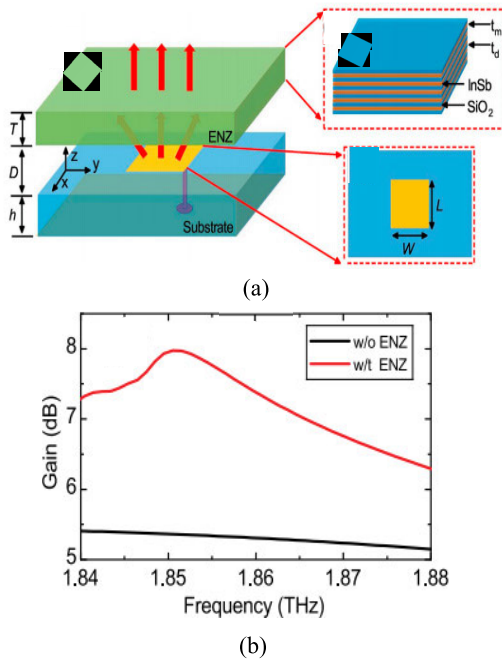
FIGURE 12. Patch antenna with multi-layer of ENZ based of [66]: (a) the configuration MTM antenna, and (b) the antenna gain with and without ENZs.
