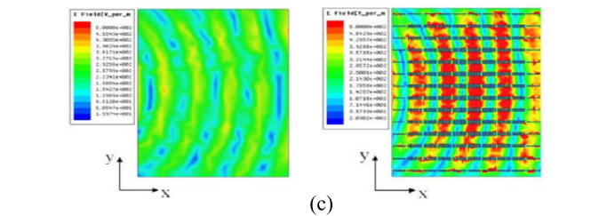
FIGURE 24. TSA with GRIN lens based of [136]: (a) the fabricated antenna with seven GRIN MTM lenses, (b) the simulated and measured gain, and (c) simulated the E-field distribution of the TSA and TSA with GRIN MTM at 10.5 GHz.
