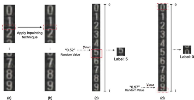
FIGURE 4. The rotating digit generator procedure. (a) The master image made by arranging the images of numbers “0” to “9” vertically. (b) The master image after applying the image inpainting technique. (c) A sample of a rotating digit generated with a random number 0.52. (d) A sample of a rotating digit generated with a random number 0.97.
