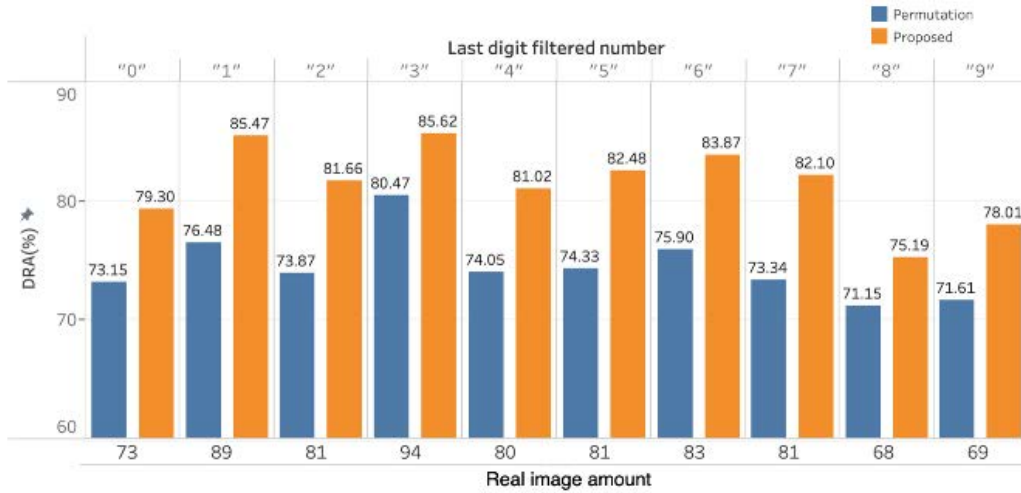
FIGURE 8. The amount of images extracted for all 10 numbers “0”~“9” and the accuracy of the models trained with the 400 images generated from the extracted images with the two augmentation methods: the proposed method (orange) and the character permutation method [15] (blue).
