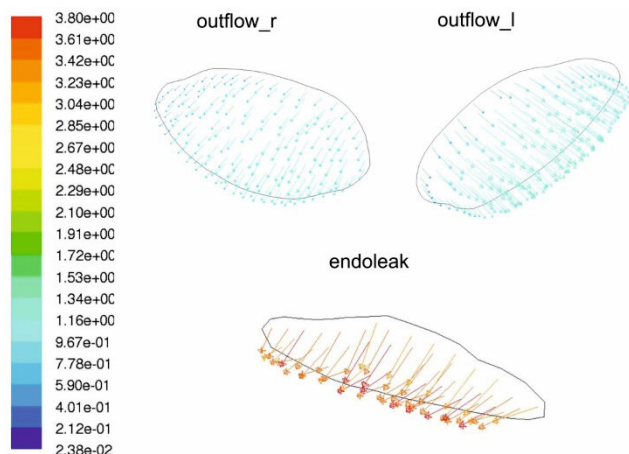
FIGURE 9. An example of velocity distribution for both outflows of both bifurcated part of the stent-graft and for the endoleak (time step 0.08s).
