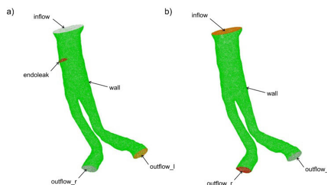
FIGURE 4. Boundary types for the stent-graft a) with the endoleak, b) without the endoleak.
