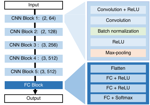
(a, b) indicates the number of convolution layer and output channel, respectively.
