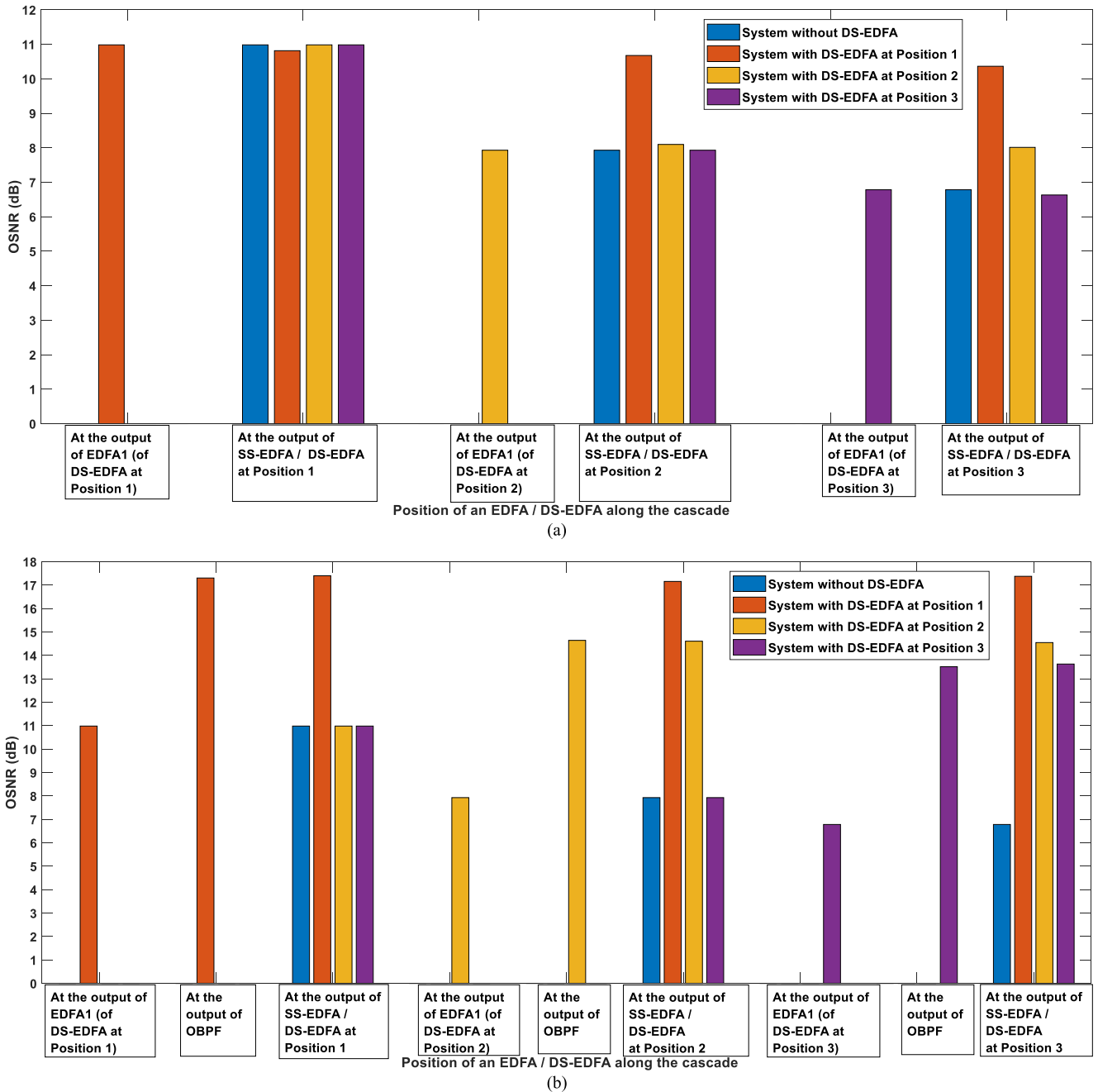
FIGURE 6. OSNR at the output of different SS-EDFAs and DS-EDFA in the cascade (a) without interstage OBPF and (b) with interstage OBPF, for P_{avTX} = -20dBm .
