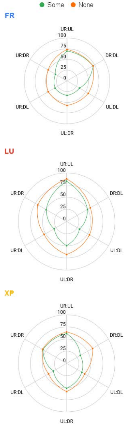
FIGURE 11. Percentage of consistent estimates for various camera locations for the specified systems in the Ekman model versus moustache occlusion.
