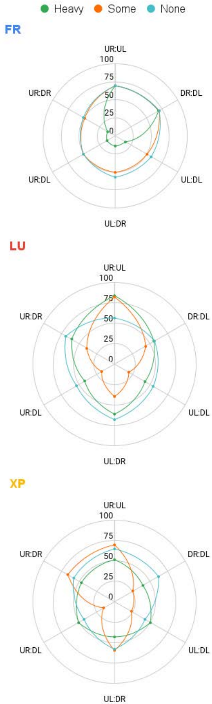
FIGURE 10. Percentage of consistent estimates for various camera locations for the specified systems in the Ekman model versus beard occlusion.
