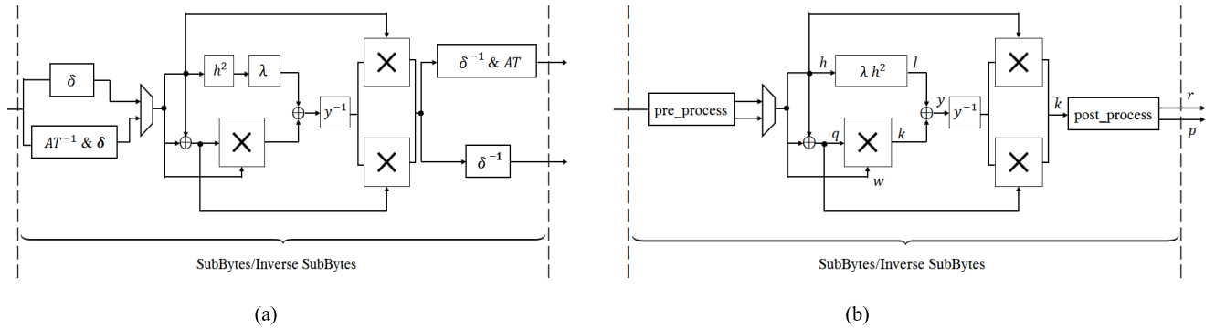
FIGURE 1. Architectures of SubBytes and inverse SubBytes operations, (a) conventional and (b) proposed approaches.
