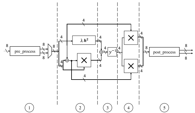
FIGURE 4. Five-stage pipelined joint S-box and inverse S-box.
