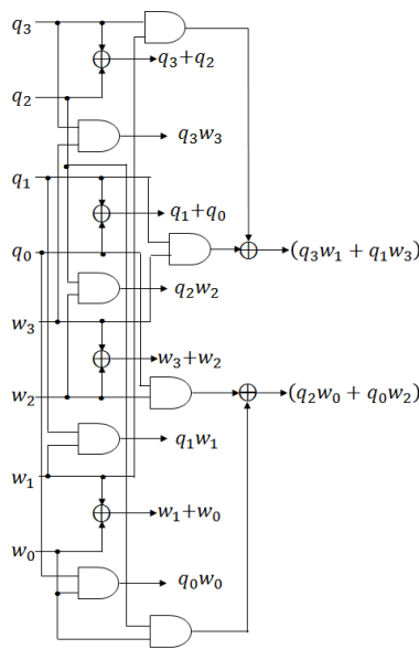
FIGURE 2. The schematic of proposed multiplication in GF((2^2)^2) .
