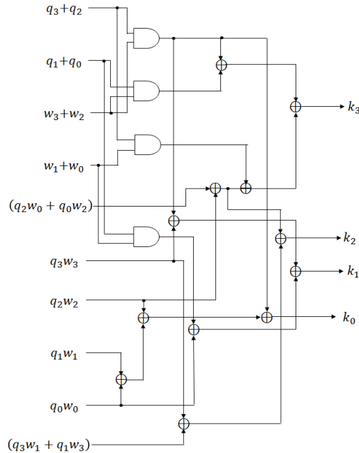
FIGURE 2. The schematic of proposed multiplication in GF((2^2)^2) .
