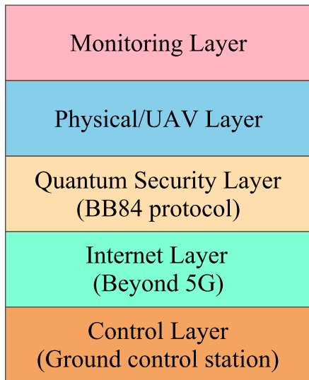
FIGURE 5. The proposed layered architecture.
