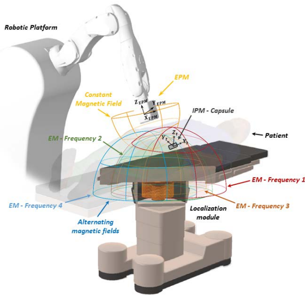
FIGURE 2. General overview of the tele-operated robotic endoscopic platform with details of the endoscopic capsule with the internal permanent magnet (IPM), and of the magnetic field distributions generated by both the external permanent magnet (EPM) and four electromagnetic (EM) sources operating at different frequencies.
