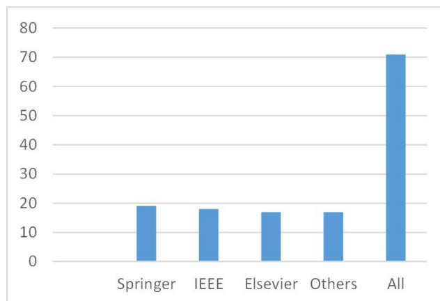
FIGURE 9. Publication venues.
