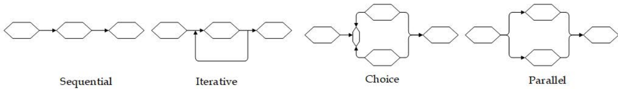
FIGURE 3. Composition Modes.
