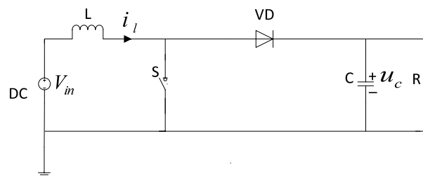
FIGURE 2. Boost converter circuit.
