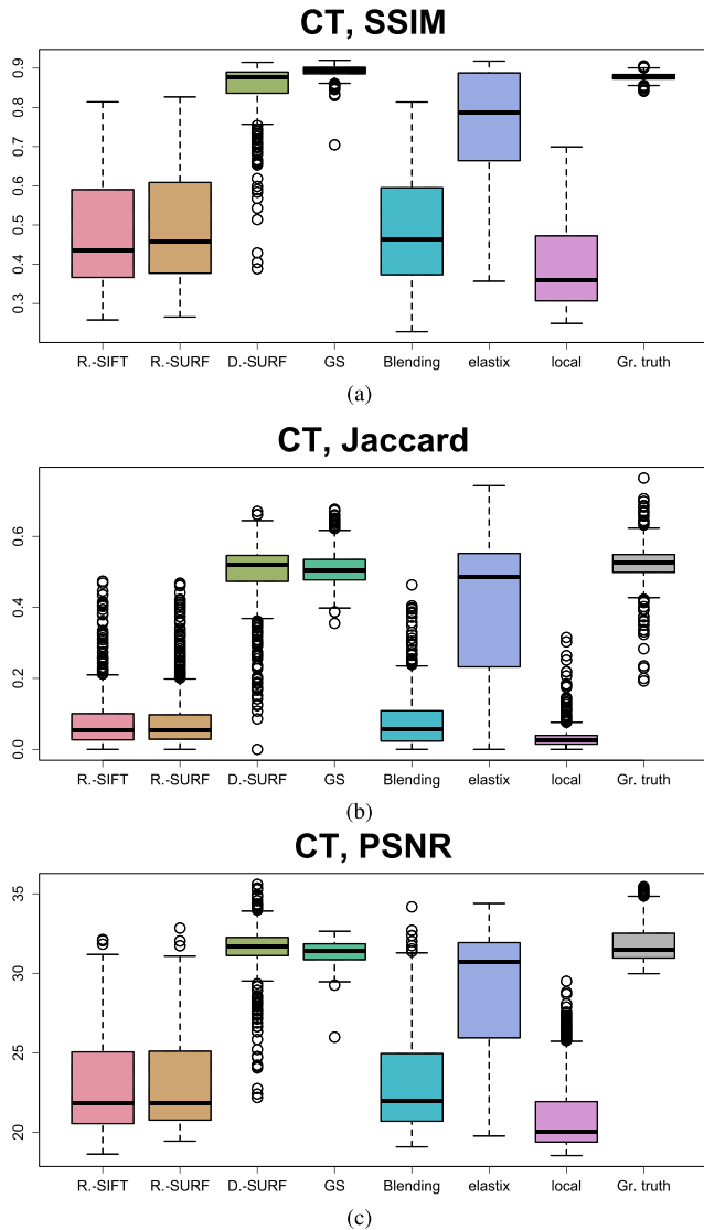
FIGURE 8. Box plots of quality measures for the CT data set. “R.-SIFT” stands for Rigid-SIFT, “R.-SURF” for Rigid-SURF, “D.-SURF” stands for Deform-SURF, “local” means local distortions only, without a global rigid transformation, “Gr. truth” stands for ground truth.
