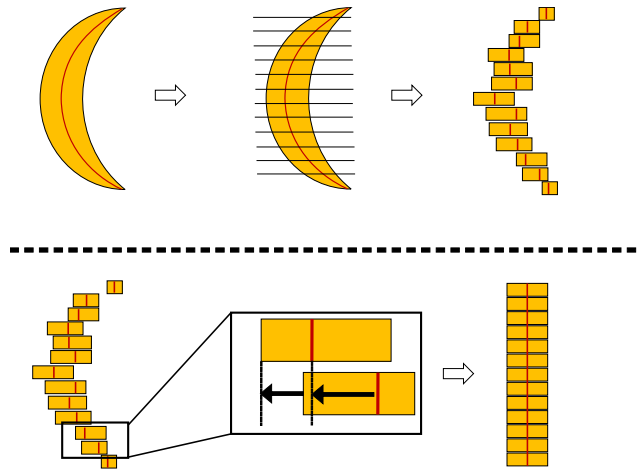
FIGURE 7. An illustration of the “banana problem”. An attempt to maintain better similarity to the neighbors produces too large distortions, destroying the originally present curvature.
