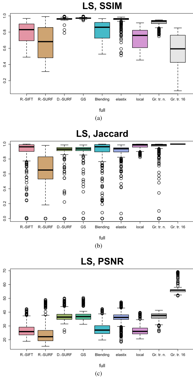
FIGURE 10. Box plots of quality measures for the LS data set. “R-SIFT” stands for Rigid-SIFT, “R-SURF” for Rigid-SURF, “D-SURF” for Deform-SURF, “local” for only local distortions, “Gr. tr. n.” for “ground truth, normalized”, “Gr. tr. 16” for “ground truth, 16 bit”. Fig. 11 shows some further details.
