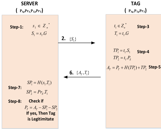
FIGURE 2. Tag authentication phase.
