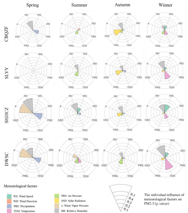
FIGURE 5. Seasonal and spatial causality between individual meteorological factors and PM2.5 concentrations for different stations.
