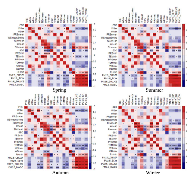
FIGURE 4. Seasonal correlations between individual meteorological factors and PM2.5 concentrations for different stations. **Correlation is significant at the 0.01 level (2 tailed); *Correlation is significant at the 0.05 level (2 tailed). Red squares show positive correlations, and blue squares show negative correlations.
