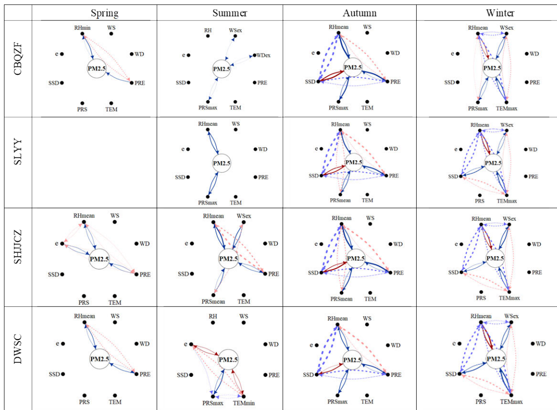
FIGURE 6. Seasonal and spatial coupling between individual meteorological factors and PM2.5 concentrations for different stations. Red represents a positive influence, and blue represents a negative influence. The solid line arrows show the causality between meteorological factors and PM2.5, while the dotted line arrows show the causality between meteorological factors. Two-way arrows show bidirectional causality, and one-way arrows show unidirectional causality. The thickness of the line arrows indicates the proportional size of the \rho value.
