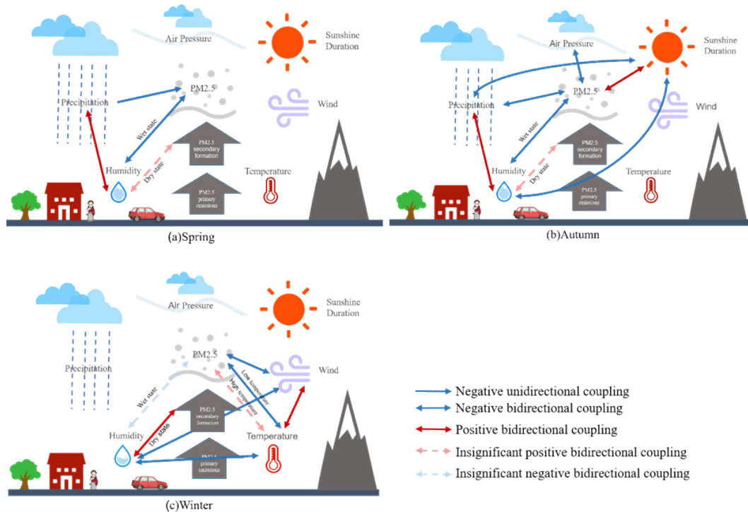
FIGURE 7. (a) Coupling pattern of meteorological factors and PM2.5 concentration in spring. (b) Coupling pattern of meteorological factors and PM2.5 concentration in autumn. (c) Coupling pattern of meteorological factors and PM2.5 concentration in winter.
