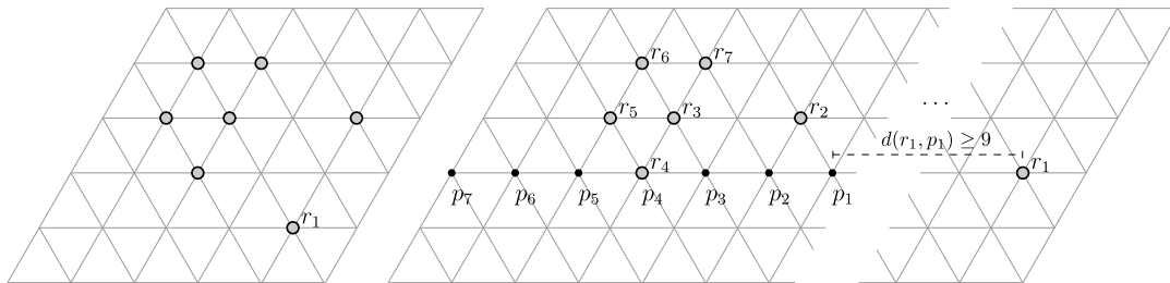
FIGURE 7. (left) An input configuration C for the LF problem. (right) The configuration C' obtained by \mathcal{A}_{LF-} at the end of the first task (Reference System).
