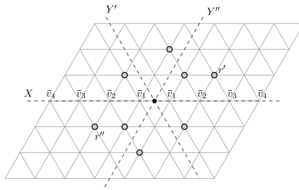
FIGURE 6. A rotational configuration C \in \mathcal{C}_0 . Here, q(\bar{C}') = (3, 11210) and q(\bar{C}'') = (2, 12200) . Since q(\bar{C}') > q(\bar{C}'') , then X and Y \equiv Y' can be used as two unoriented axes. In the obtained reference system, the equivalent robots r' and r'' are both in position (3, 1) .
