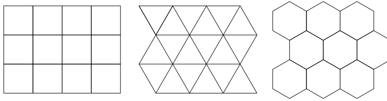
FIGURE 2. Part of regular plane tessellations.
