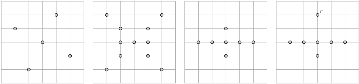
FIGURE 3. Representation of some initial configurations defined on G_5 : from left to right, in the text they are referred as C_1 , C_2 , C_3 , and C_4 .
