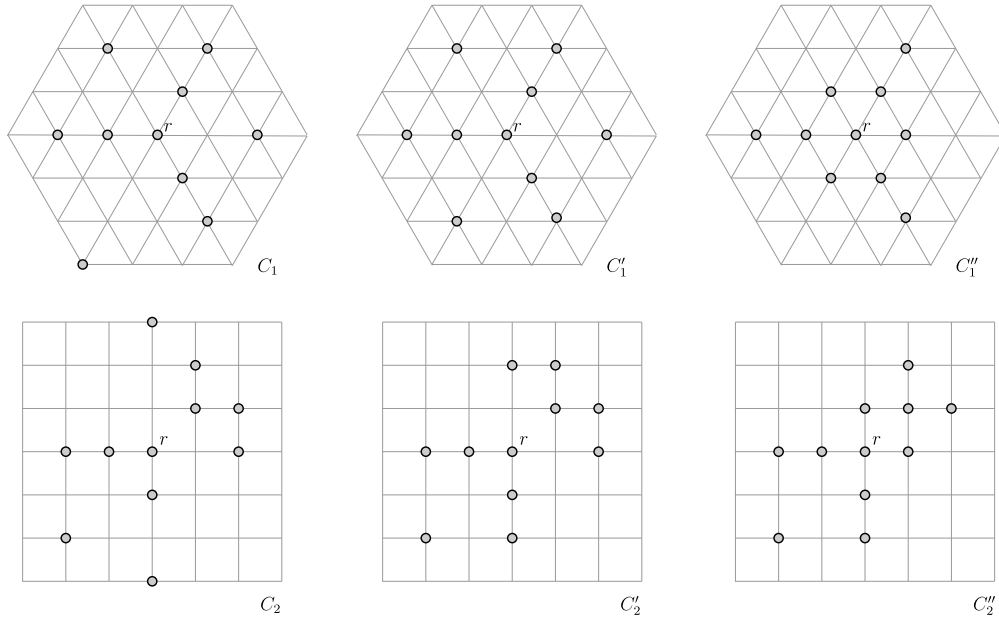
FIGURE 5. C_1 is almost-rotational (cf. Definition 6) and C_2 is almost-diagonal (cf. Definition 8). Notice that C'_1 = Reduce(C_1, r) and C''_1 = Compact(C'_1, r) = Compact(C_1, r) ; moreover, C'_2 = Reduce(C_2, r) and C''_2 = Compact(C'_2, r) = Compact(C_2, r) .
