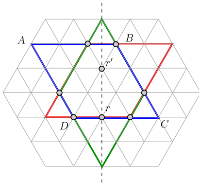
FIGURE 4. Visualization of some notation used in the paper. An initial reflective configuration C defined on G_T : circles represent robots. It shows the three possible bounding parallelograms. They have all the same size. LSS(R) = 0011000111011010 and it is generated in both the red and blue parallelograms. In the blue one, LSS(R) is generated from corner A along the side AD . Robot r is the pivot of C .
