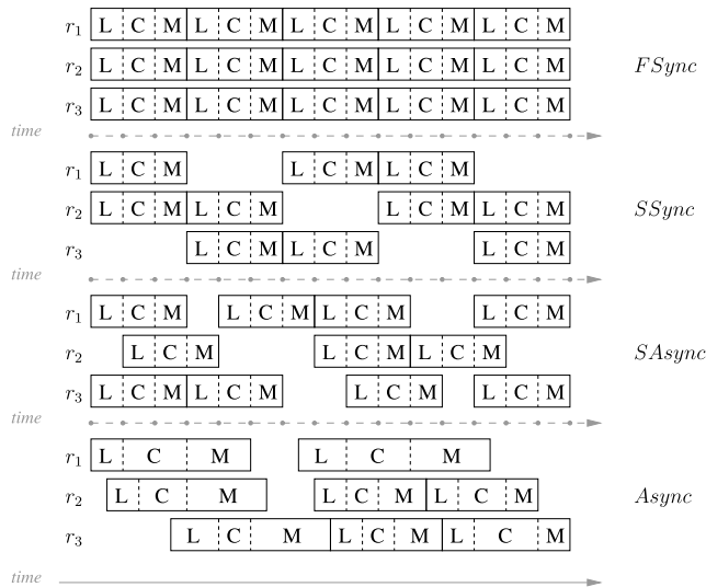
FIGURE 1. The execution model of computational cycles for each of FSync, SSync, SASync, and Async robots. The inactivity of robots is implicitly represented by empty time periods.
