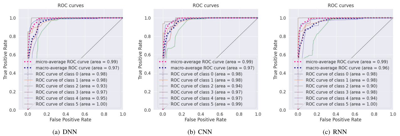
FIGURE 15. The Receiver Operating Characteristic (ROC) curves for MQTTset datasets. (class 0: Bruteforce, class 1: DoS, class 2: Flood, class 3: Benign, class 4: Slowlite, class 5: Malformed.)
