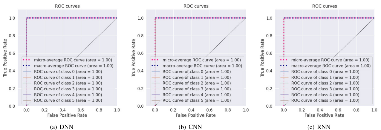
FIGURE 16. The Receiver Operating Characteristic (ROC) curves for TON_IOT dataset. (class 0: Backdoor, class 1: Injection, class 2: Benign, class 3: Password, class 4: Scanning, class 5: XSS.)
