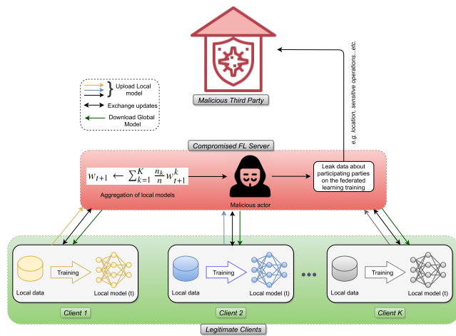
FIGURE 11. Privacy leakage attack in federated learning.
