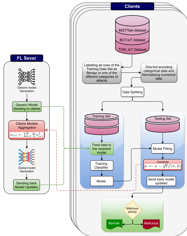
FIGURE 12. The architecture of our federated deep learning-based IoT intrusion detection system.
