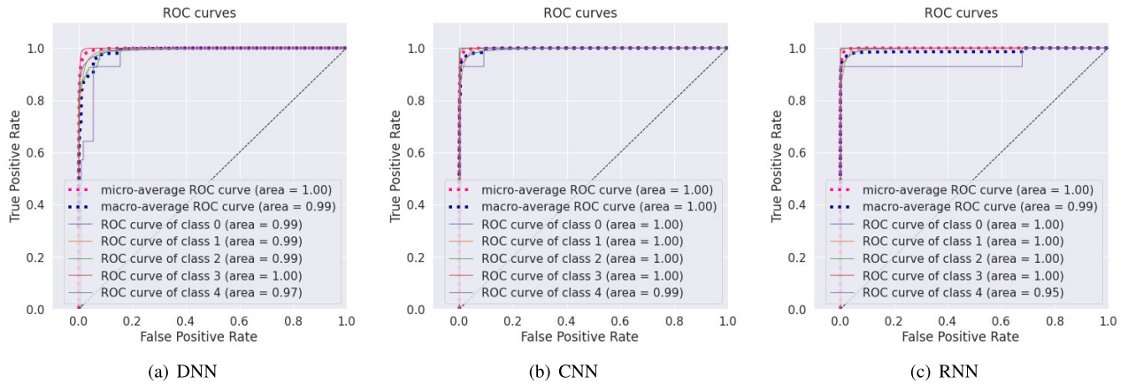
FIGURE 14. The Receiver Operating Characteristic (ROC) curves for BoT-IoT dataset. (class 0: DDoS, class 1: DoS, class 2: Benign, class 3: Reconnaissance, class 4: Theft.)
