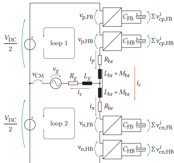
FIGURE 4. Equivalent circuit of one phase of a hybrid MMC, where all the SMs are presented as two units, being equivalent to the clusters of the installed FB and HB SMs. The following notation is applied: C_{FB} , C_{HB} – equivalent capacitance of all SMs within FB and HB, respectively; \Sigma v_{c\{p,n\},FB}^i , \Sigma v_{c\{p,n\},HB}^i – total available capacitor voltage of the corresponding clusters, v_{\{p,n\},FB} , v_{\{p,n\},HB} – total inserted voltage of the corresponding SM clusters.
