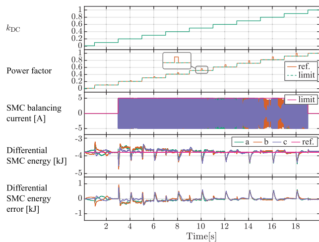
FIGURE 17. SMC balancing action for the second test scenario. Differential energy divergence is seen successfully controlled after each k_{DC} step. However, power factor alteration above the limit causes sharp SMC energy deviation, at t \in \{4 \text{ s}, 6 \text{ s}, \dots, 18 \text{ s}\} instants. Operation in prohibited area would thus quickly drive the converter out of operation by overcharging FB- and fully discharging HB SMs, or vice versa. One can notice power factor deviation at k_{DC} = 0.1 has no impact, as this is the area of FB-only operation capability (see Fig. 15).
