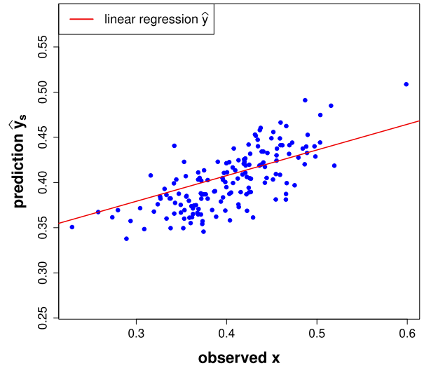
FIGURE 11. \hat{y}_s(j) predictions for 159 batters using \mathcal{P}_{5,10} partition and LR line.
