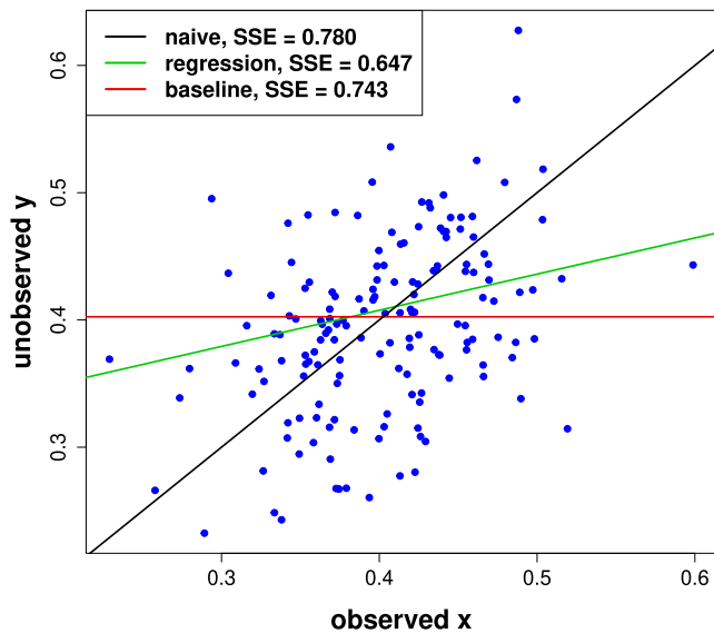
FIGURE 2. (x(j), y(j)) points with naive, regression, and baseline predictions.
