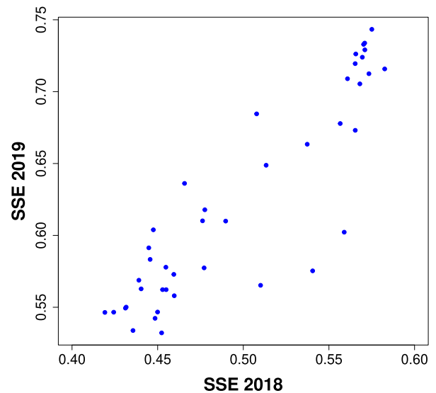
FIGURE 4. Prediction SSE in 2018 and 2019 for 42 partitions.
