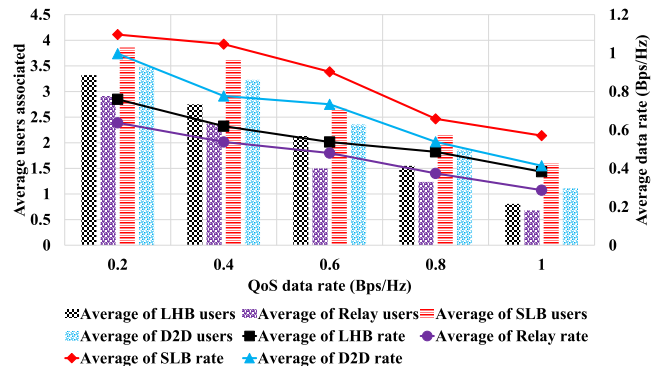
FIGURE 6. Users association-data rate versus QoS requirements using DU-CPL access in the UL.
