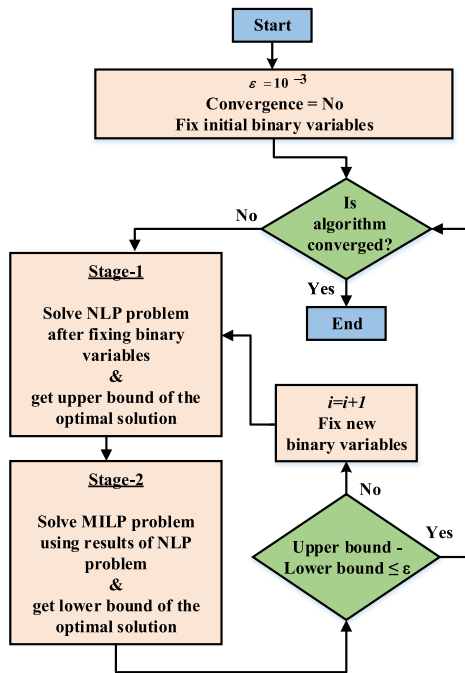
FIGURE 2. Flow chart - \epsilon -optimal algorithm.
