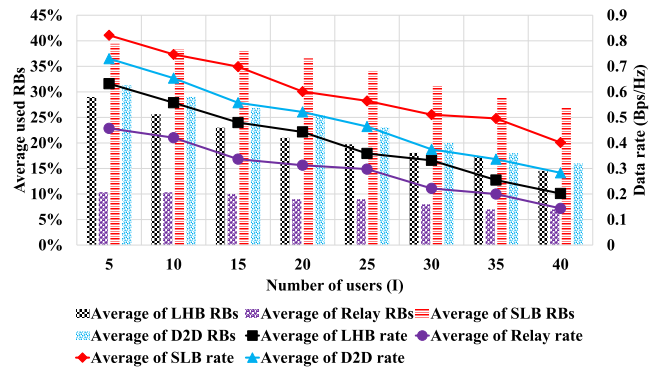
FIGURE 10. RBs-data rate versus QoS requirements using DU-CPL access in the UL.
