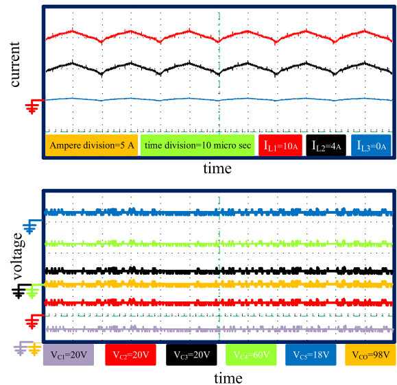
FIGURE 15. The experimental results of the inductors current and capacitors voltage.
