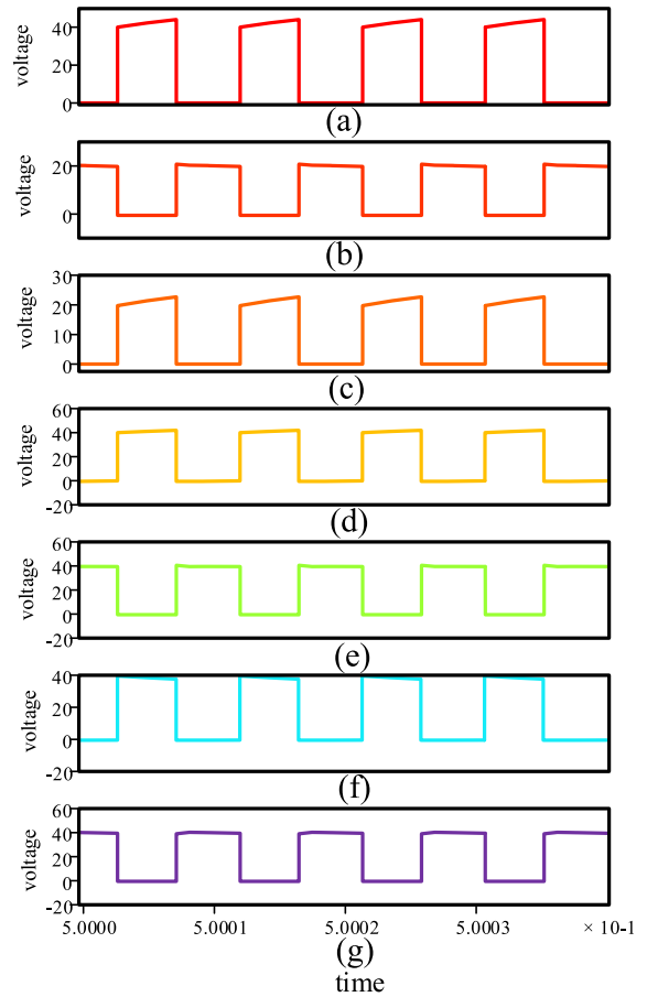
FIGURE 14. The simulation results: (a) the first switch voltage, (b) the first diode voltage, (c) the second diode voltage, (d) the third diode voltage, (e) the fourth diode voltage, (f) the fifth diode voltage, and (g) sixth diode voltage.
