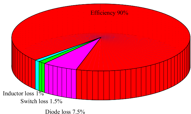
FIGURE 22. The pie chart of the experimental efficiency and power losses.
