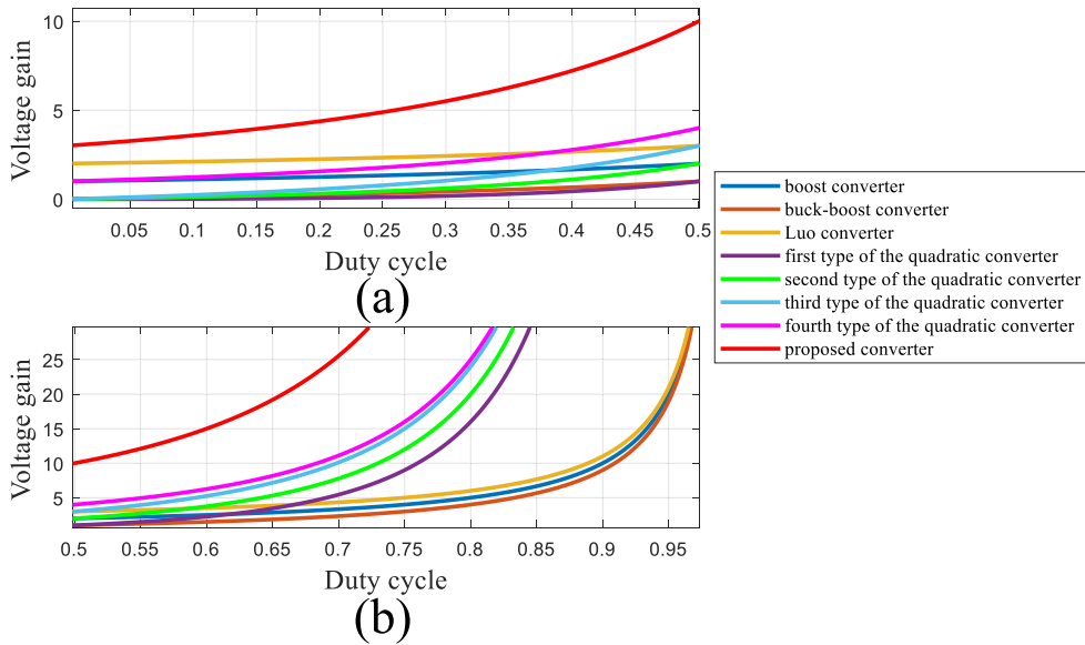
FIGURE 3. The comparison of the ideal voltage gain of the suggested design with the boost, buck-boost, Luo, and four types of the quadratic converters.
