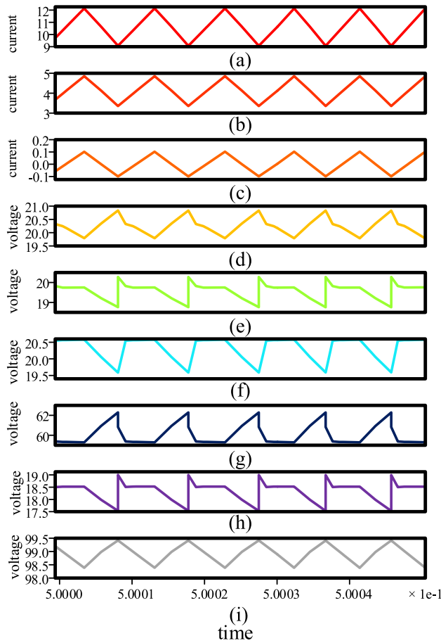
FIGURE 11. The simulation results: (a) the first inductor current, (b) the second inductor current, (c) the third inductor current, (d) the first capacitor voltage, (e) the second capacitor voltage, (f) the third capacitor voltage, (g) the fourth capacitor voltage, (h) the fifth capacitor voltage, and (i) output voltage.
