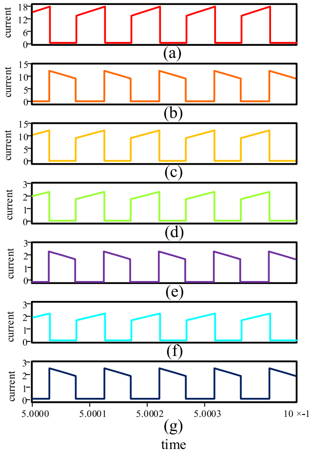
FIGURE 13. The simulation results: (a) the first switch current, (b) the first diode current, (c) the second diode current, (d) the third diode current, (e) the fourth diode current, (f) the fifth diode current, and (g) sixth diode current.
