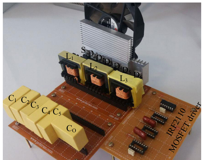
FIGURE 19. The prototype.
