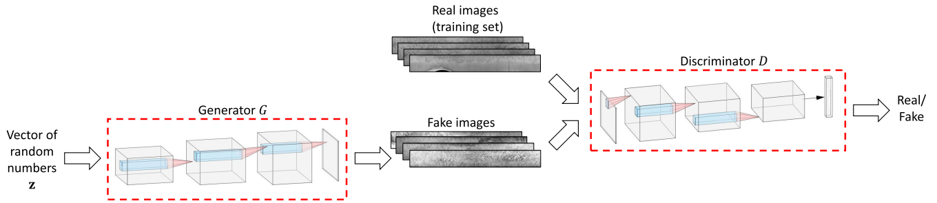
FIGURE 7. Architecture of the deep convolutional GAN (DCGAN) used in this work. To train the generator G and the discriminator D , we use a database of RSMs of irises. The generation process is performed by applying G on a vector \mathbf{z} composed by random numbers in the range [0, 1] , extracted following a normal distribution.
