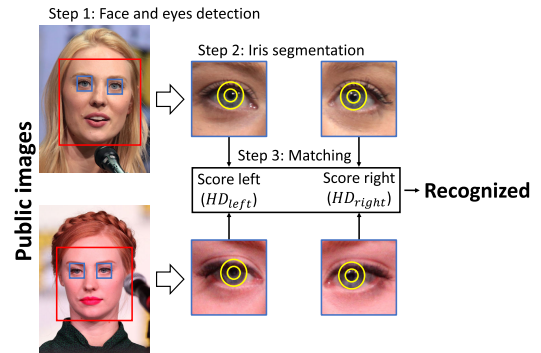
FIGURE 2. Outline of the methodology used to perform iris recognition using public domain face images. It is possible to use robust methods to automatically detect the face, extract the eye positions, segment the irises, and then compare them to achieve high-confidence recognition.
