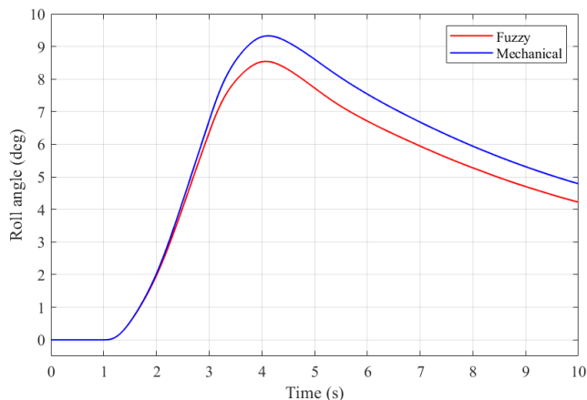
FIGURE 12. Roll angle.
