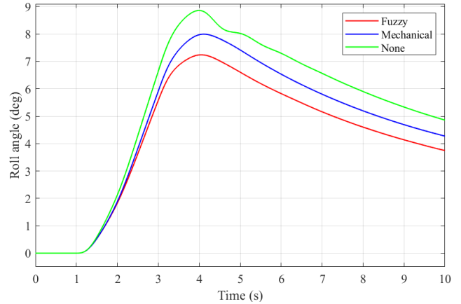
FIGURE 10. Roll angle.
