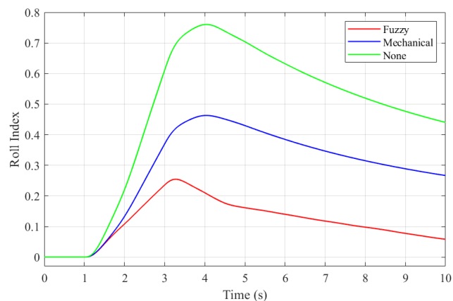
FIGURE 9. Roll index.
