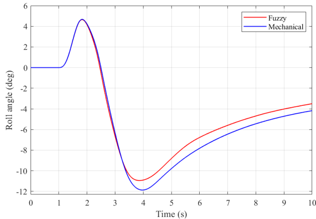
FIGURE 18. Roll angle.
