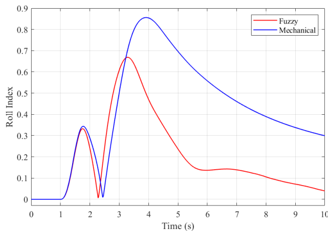
FIGURE 19. Roll index.
