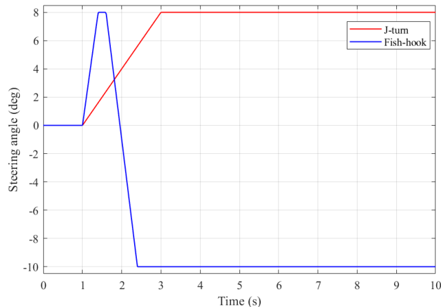
FIGURE 7. Steering angle.
