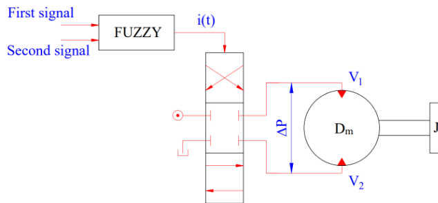
FIGURE 3. Schematic of the hydraulic motor and servo valve.
