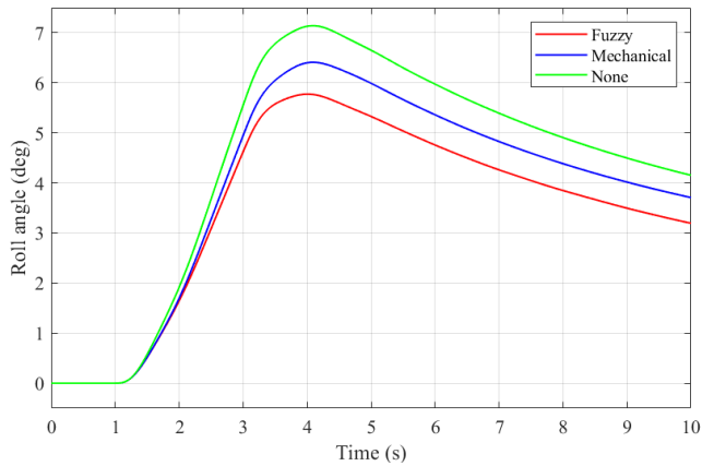
FIGURE 8. Roll angle.
