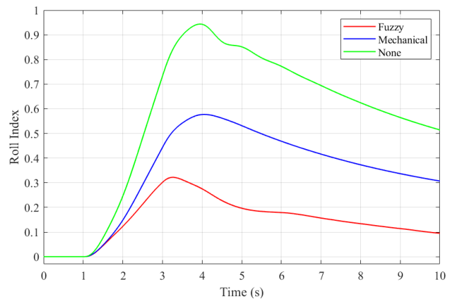
FIGURE 11. Roll index.
