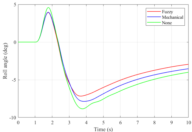
FIGURE 14. Roll angle.
