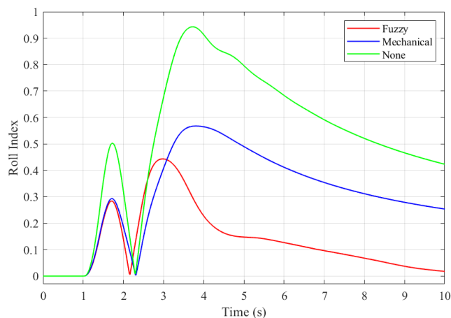
FIGURE 15. Roll index.
