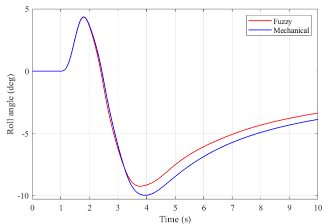
FIGURE 16. Roll index.
