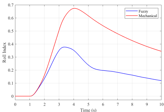
FIGURE 13. Roll index.
