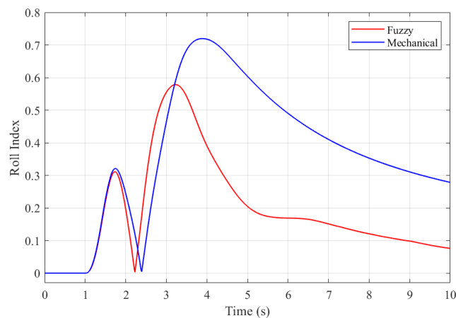
FIGURE 17. Roll index.
