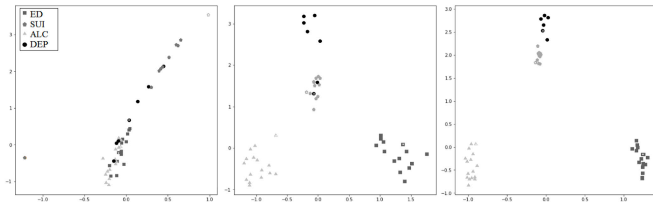
FIGURE 4. Task 1 - Vectors in two dimensions of the top 15 predictive terms of each class. The representations correspond to the 1) Word2vec baseline model (TEVP = 97%), 2) Embedding model 0 (TEVP = 72%), and 3) Embedding model 2 (TEVP = 91%). White dots are placed over pivot terms.
