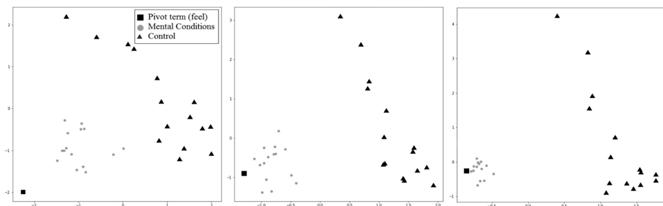
FIGURE 5. Task 2 - Vectors in two dimensions of the top 15 predictive terms of each class. The representations correspond to the 1) Word2vec baseline model (TEVP = 36%), 2) Embedding model 0 (TEVP = 48%), and 3) Embedding model 2 (TEVP = 60%). The pivot term is represented by a square.
