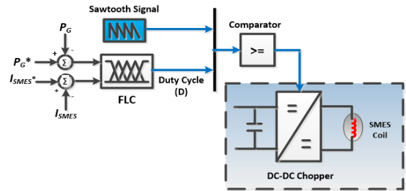
FIGURE 9. Control of dc-dc chopper using FLC.
