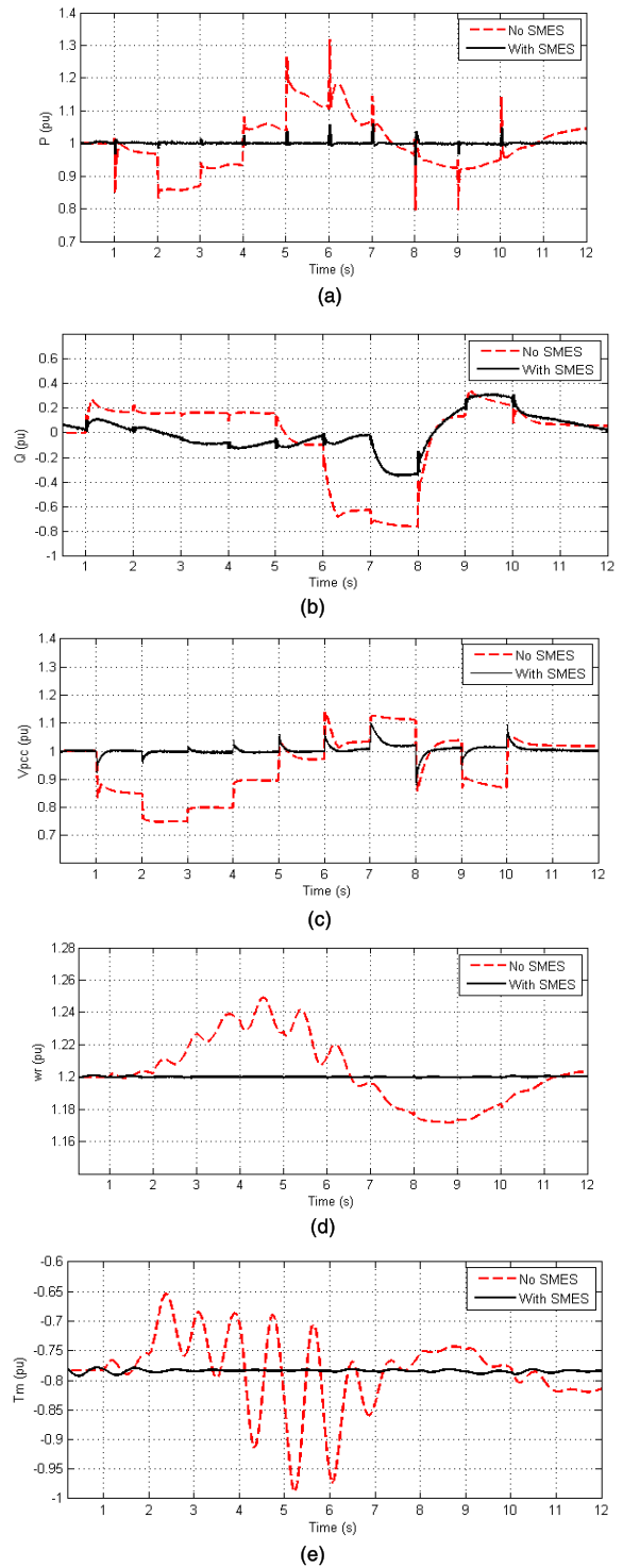
FIGURE 12. DFIG performance during grid voltage variation with and without SMES; (a) DFIG active power; (b) DFIG reactive power; (c) Voltage at PCC; (d) DFIG rotor speed; (e) DFIG electromagnetic torque.
