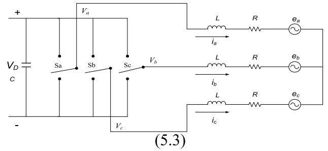
FIGURE 4. Equivalent schematic diagram of a VSC connected to the grid.
