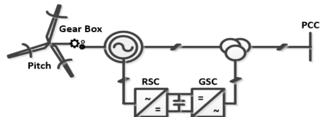
FIGURE 2. Generic model of a DFIG.
