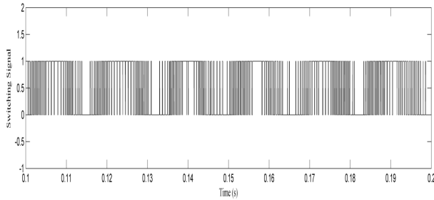
FIGURE 7. Typical switching VSC signal.
