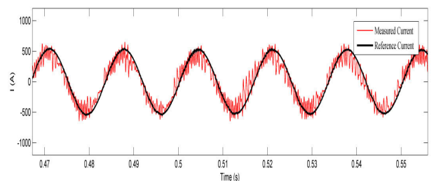
FIGURE 6. Typical hysteresis current waveform.
