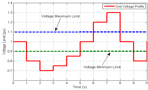
FIGURE 11. Assumed voltage profile at the weak-grid side.
