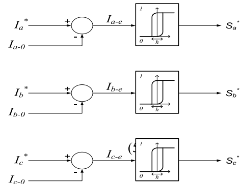
FIGURE 5. Control of VSC using HCC.
